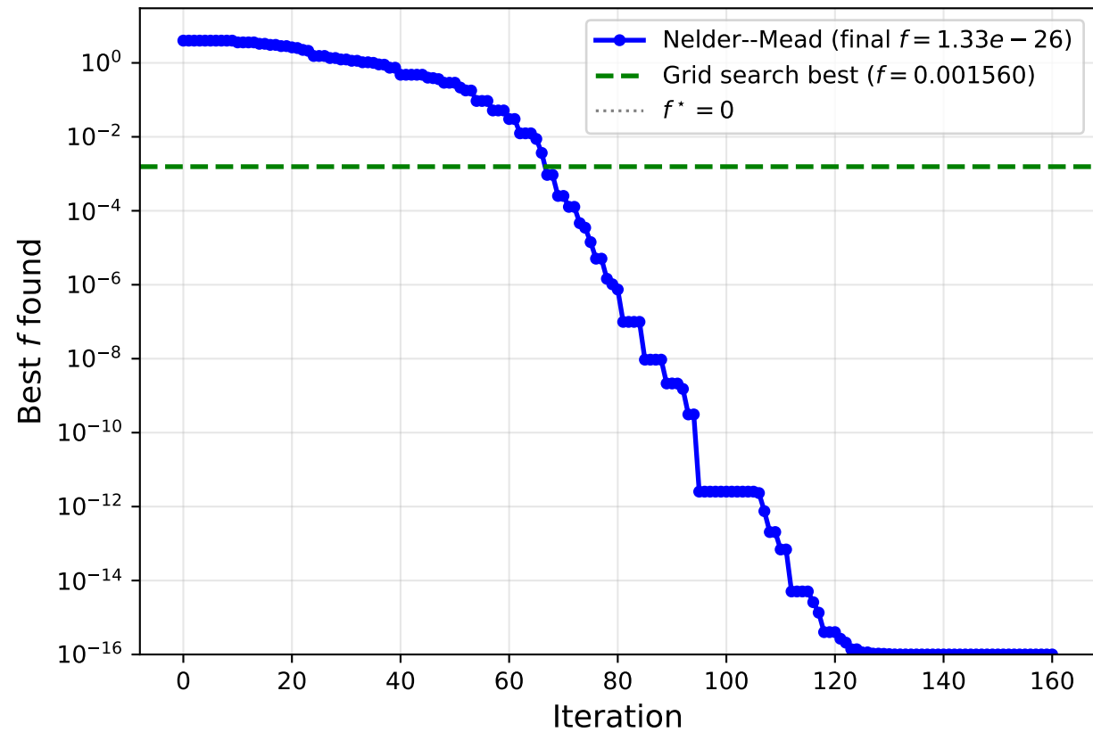
Q4B: Nelder--Mead on Benchmark C (Rosenbrock, \kappa \approx 2504 )
