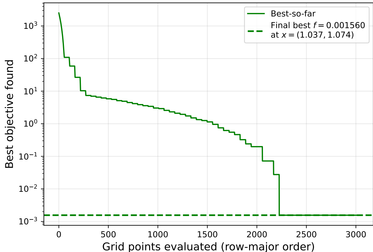
Q4B: Grid Search on Benchmark C (3025 evaluations on 55 \times 55 grid)
