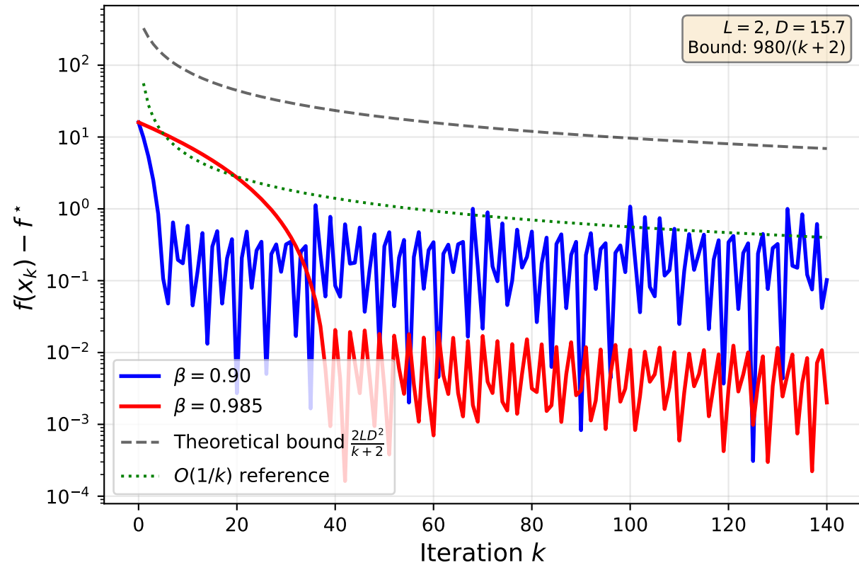
Frank--Wolfe: Interior Optimum
