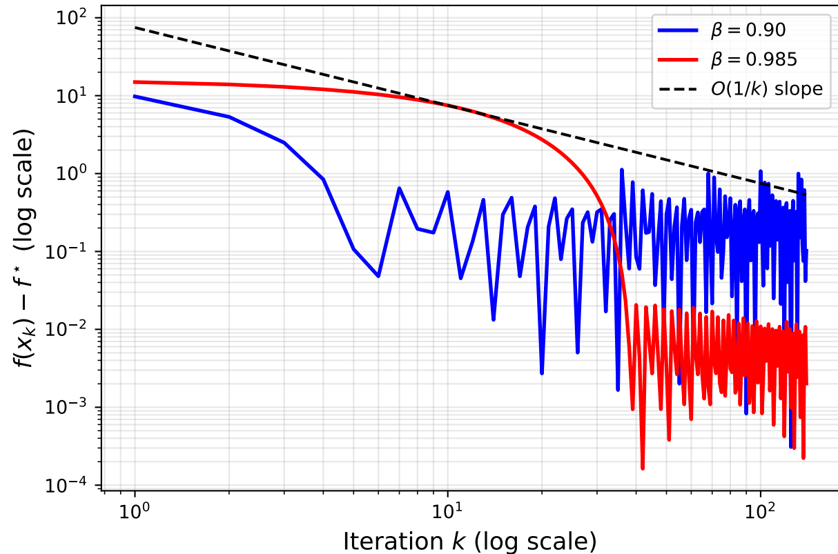
Frank--Wolfe: Log-Log Rate Verification
