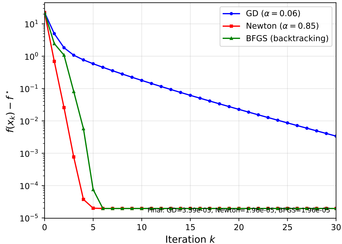
Benchmark B ( \kappa \approx 5.6 )
