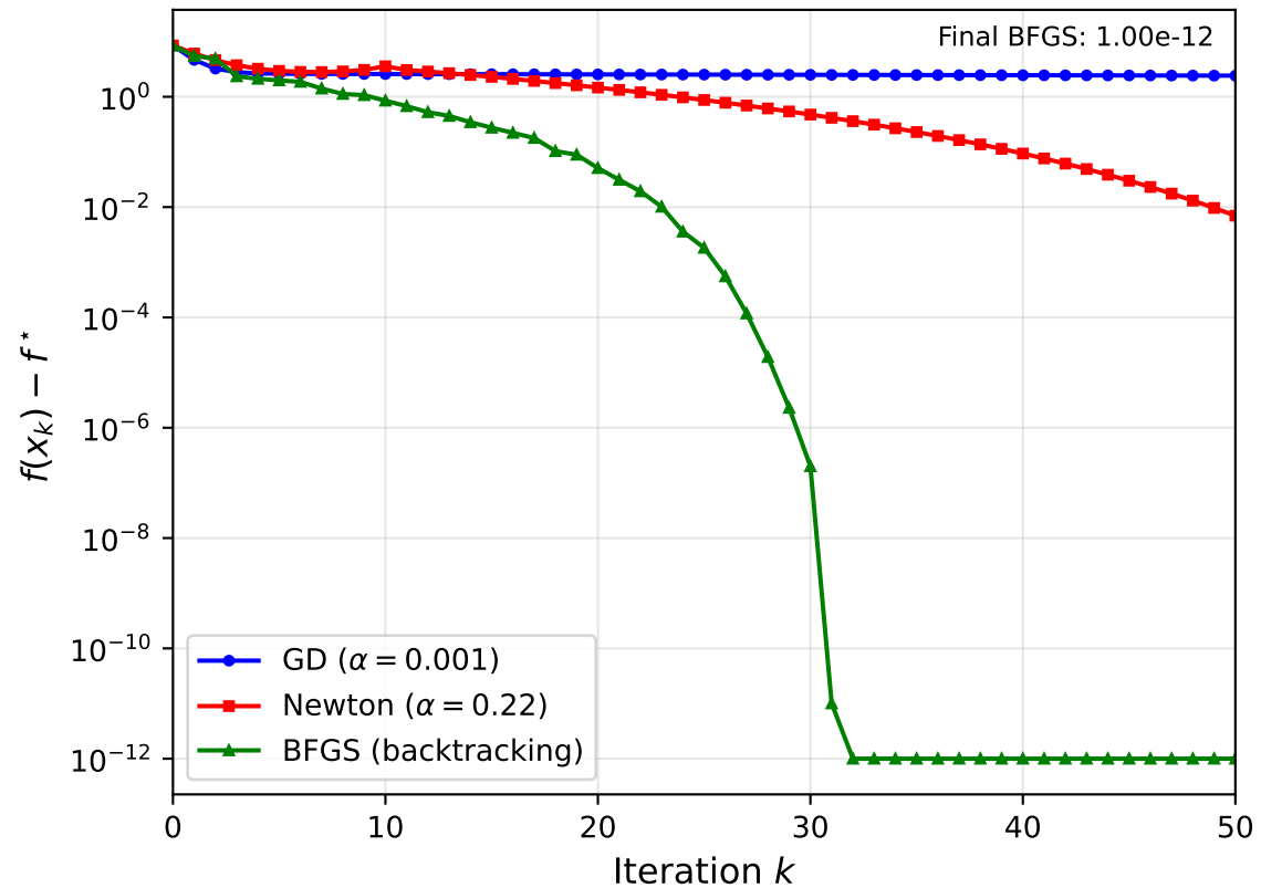
Benchmark C (Rosenbrock, \kappa \approx 2500 )
