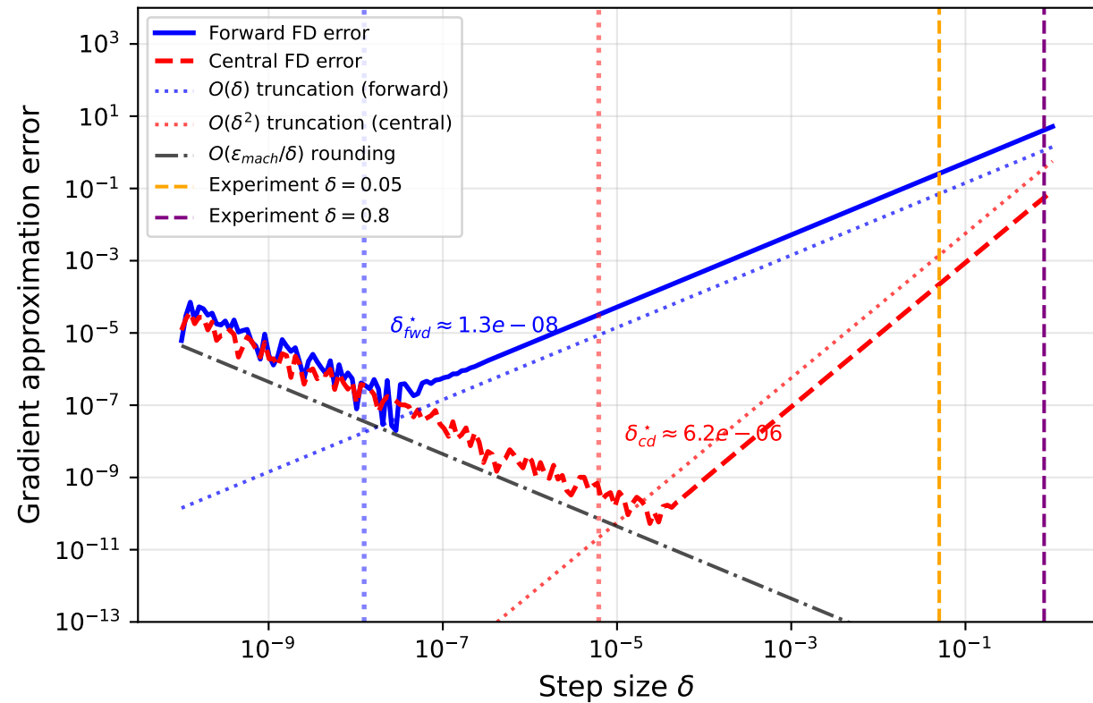
FD Gradient Error vs. \delta (Benchmark B, x_0 = (-1, 4) )
