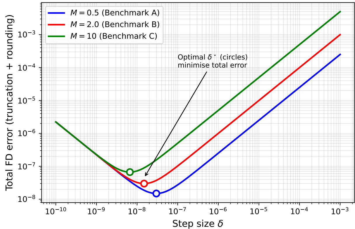
Optimal \delta Theory (Forward FD: \delta^* = \sqrt{2\epsilon_{mach}/M} )
