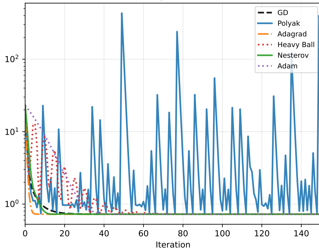
Bench. B: Toy Neural Network
