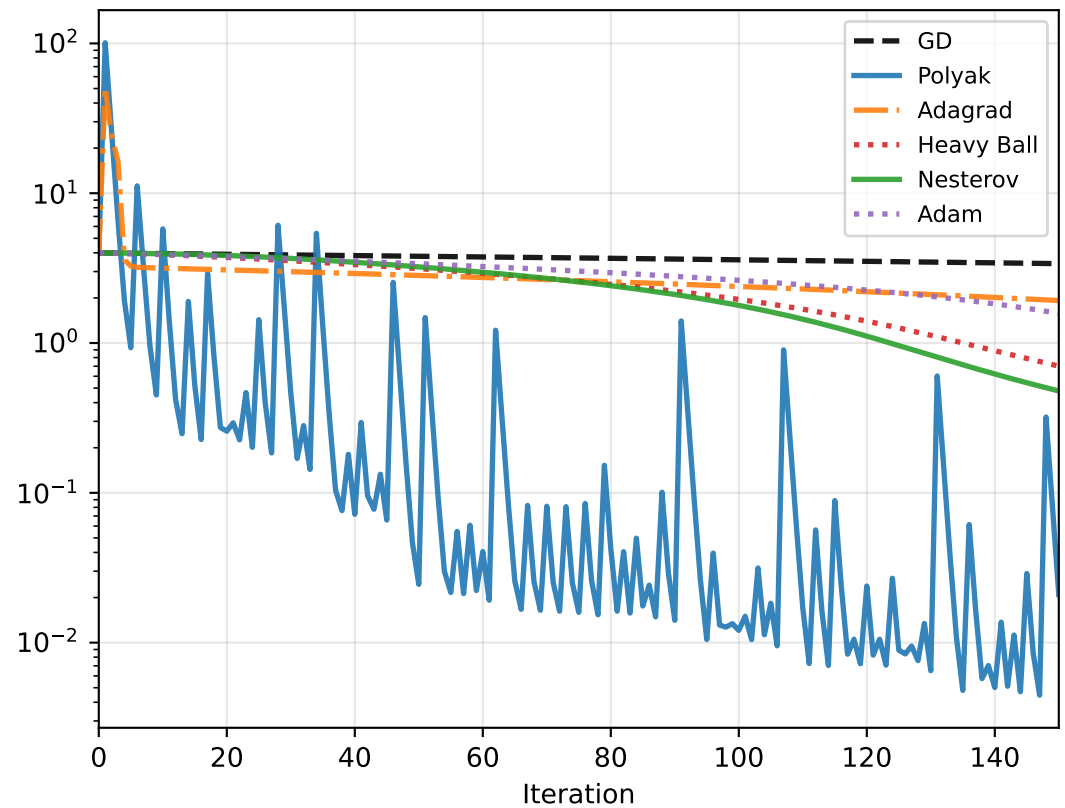
Bench. C: Rosenbrock
