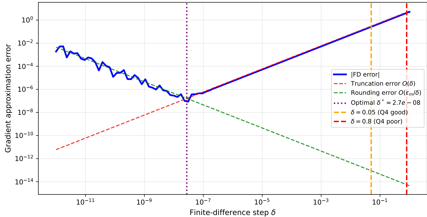
Q4: FD Gradient Error vs Step Size — Benchmark B at x_0 = (-1, 4)
