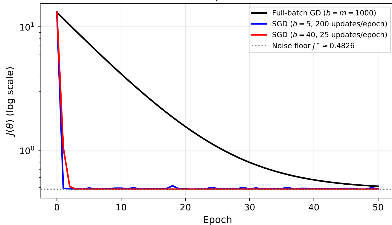
Per-Epoch Convergence (SGD with more updates dominates)
