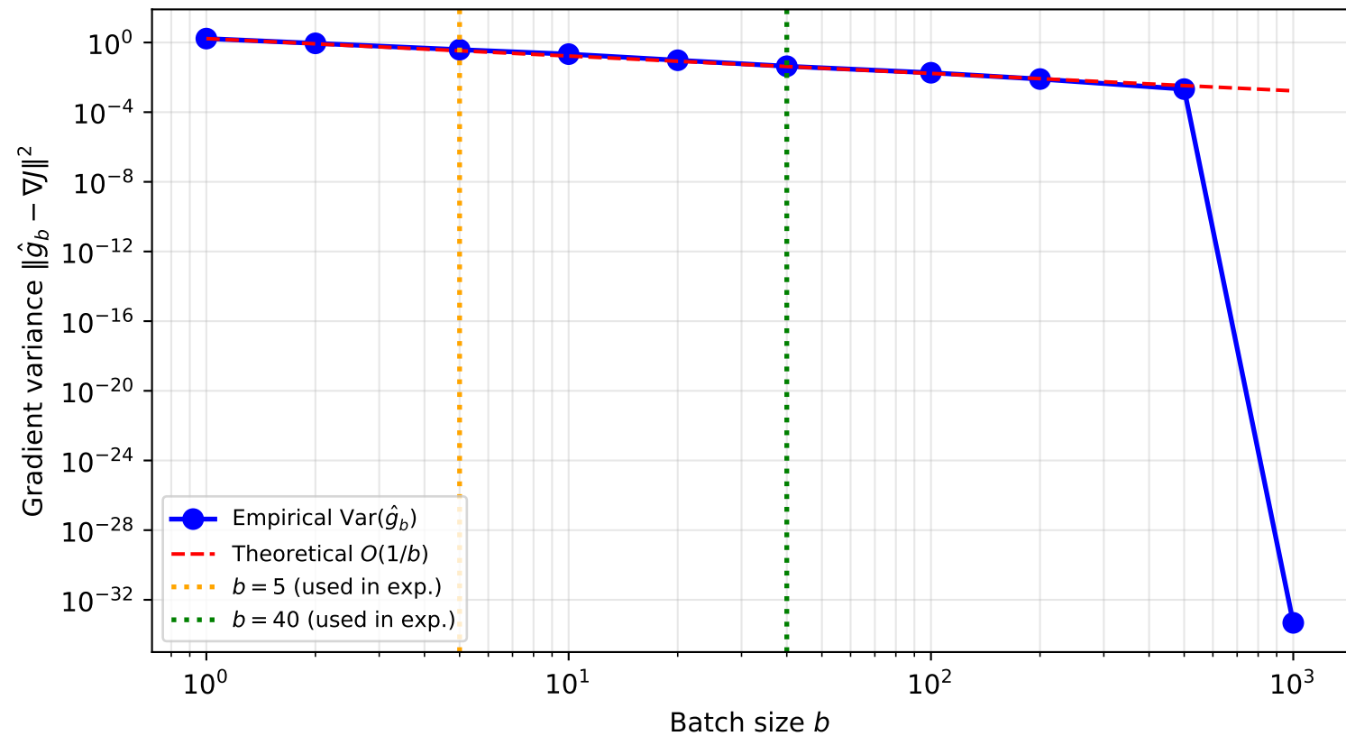
Q2: Mini-Batch SGD Gradient Variance vs Batch Size at OLS Solution \theta_{\text{OLS}}
