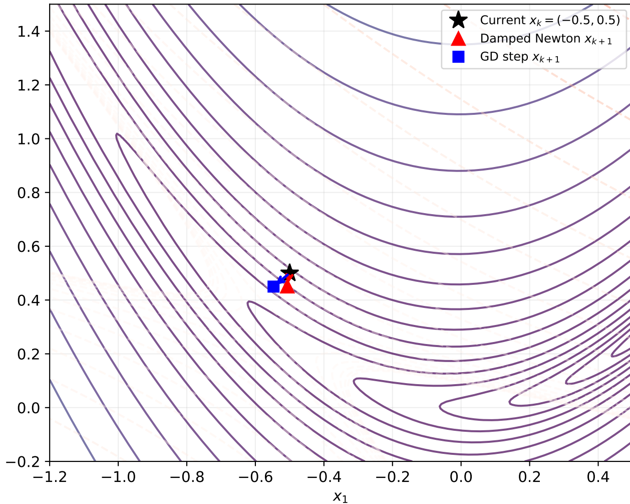
Q3: Rosenbrock Contours (solid) vs Quadratic Approx. (dashed) at (-0.5, 0.5)
