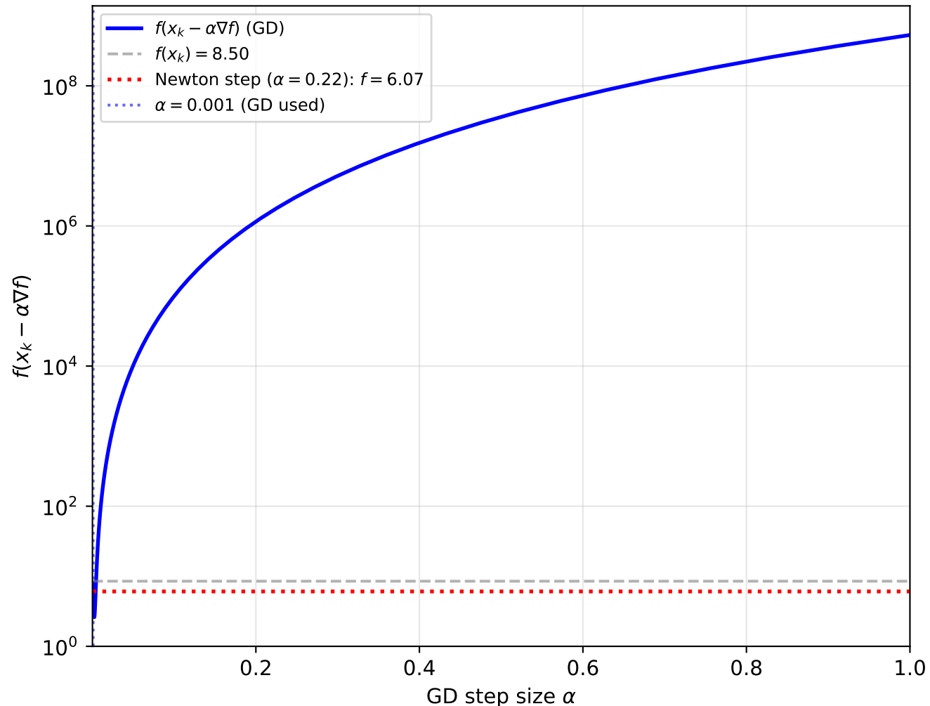
Q3: GD Step Size Sensitivity at (-0.5, 0.5) vs Newton's Single Step
