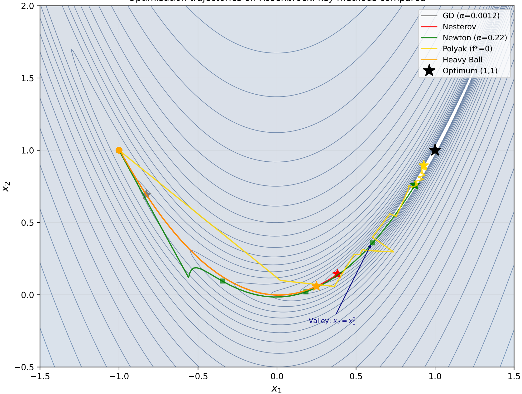
Optimisation trajectories on Rosenbrock: key methods compared
