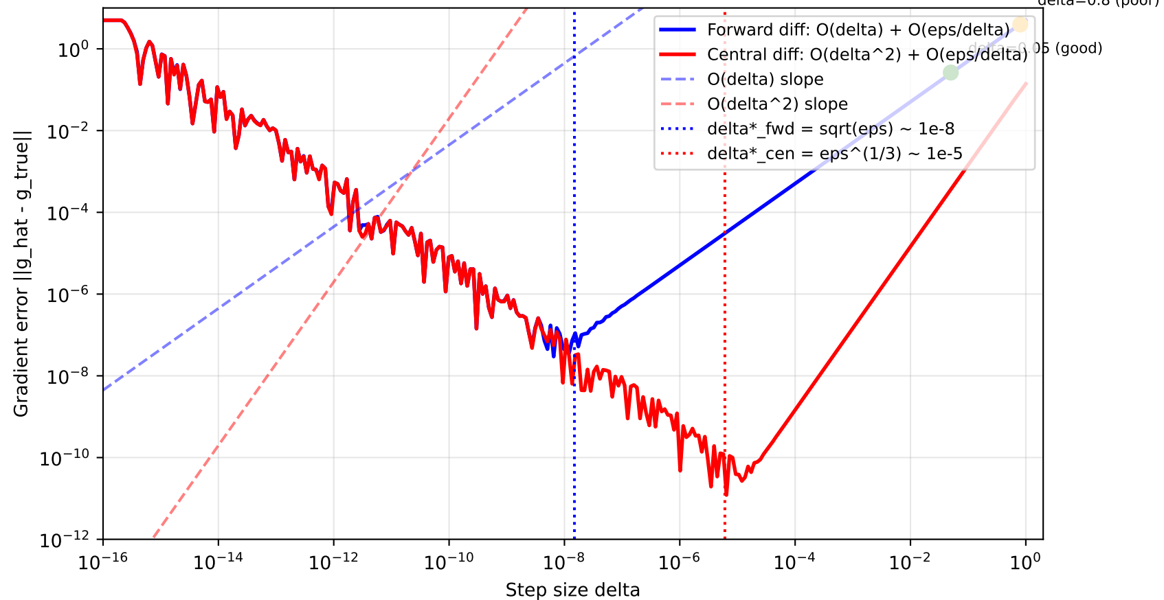
Forward vs Central Finite Difference Error (Benchmark B, x=(0.5, 2.5) )
