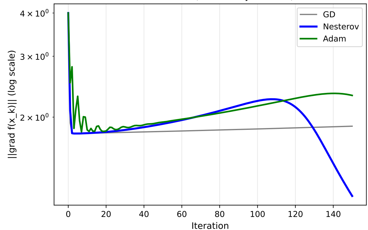
Trajectories on Rosenbrock (150 iters)
