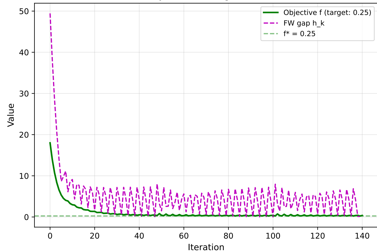
FW Boundary Case: Convergence (beta=0.93)
