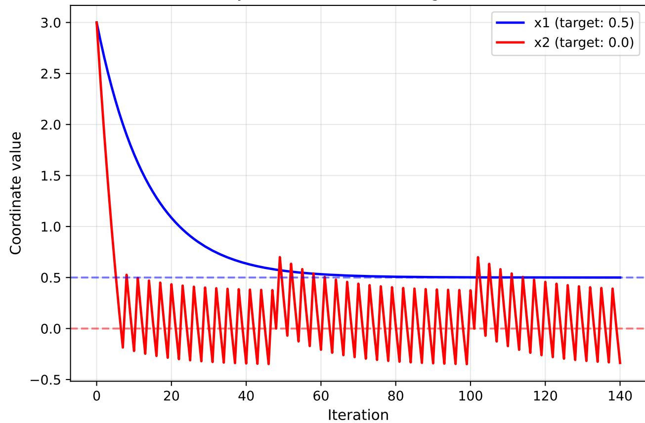
FW Boundary Case: Coordinate Convergence (beta=0.93)
