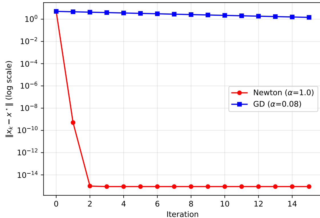
Benchmark A (Quadratic Loss) Newton vs GD: Error Convergence
