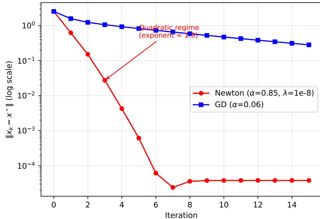
Benchmark B (Non-convex Neural Net) Newton vs GD: Error Convergence
