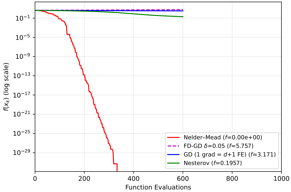
Convergence vs Function Evaluations
