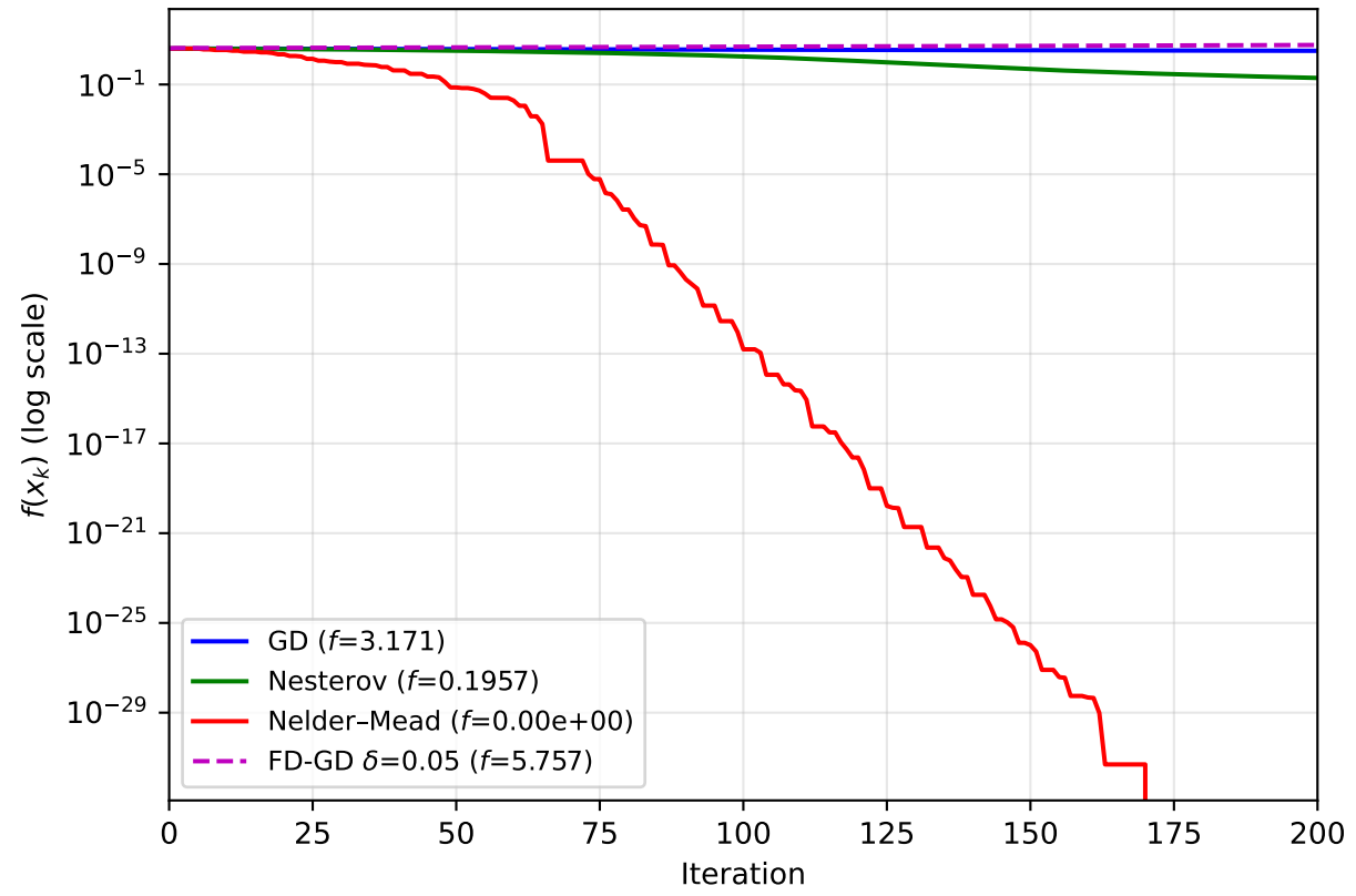
Convergence vs Iteration
