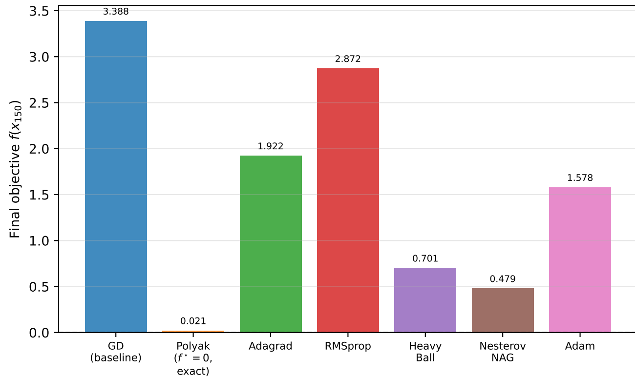
Final values after 150 iterations
