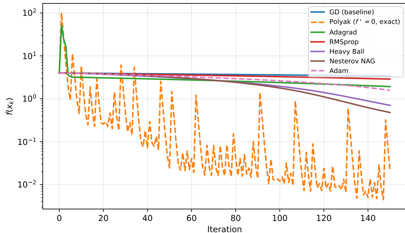
All methods: Benchmark C (Rosenbrock, \kappa \approx 2504 )
