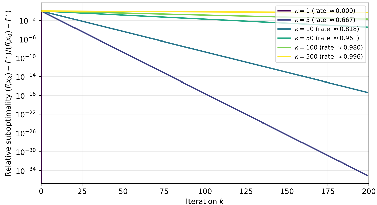
GD Convergence Rate vs. Condition Number \kappa = L/\mu (optimal fixed step \alpha = 2/(\mu + L) )
