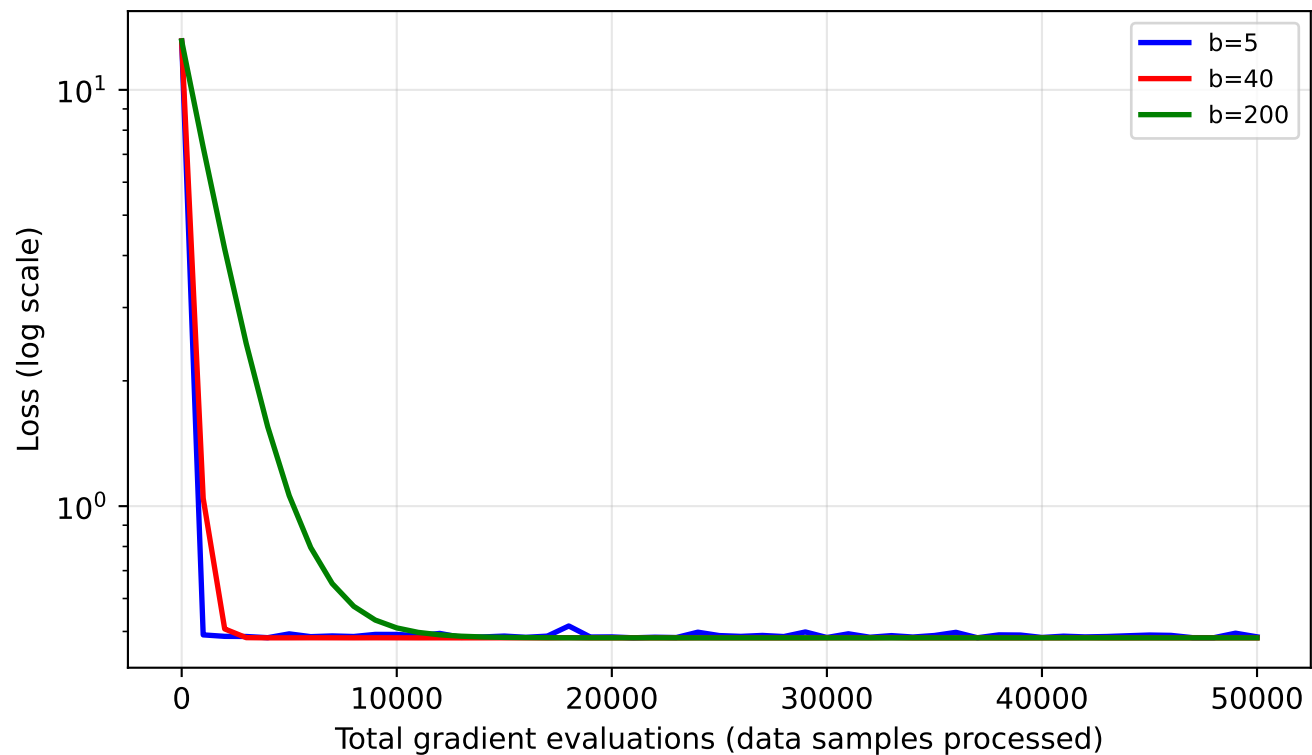
Mini-Batch SGD: Convergence per Sample (Benchmark A)
