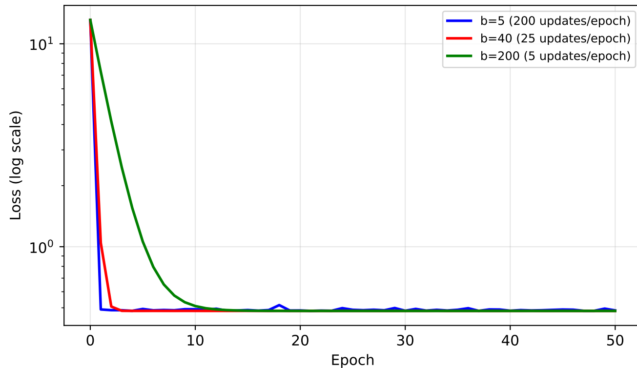
Mini-Batch SGD: Convergence per Epoch (Benchmark A)
