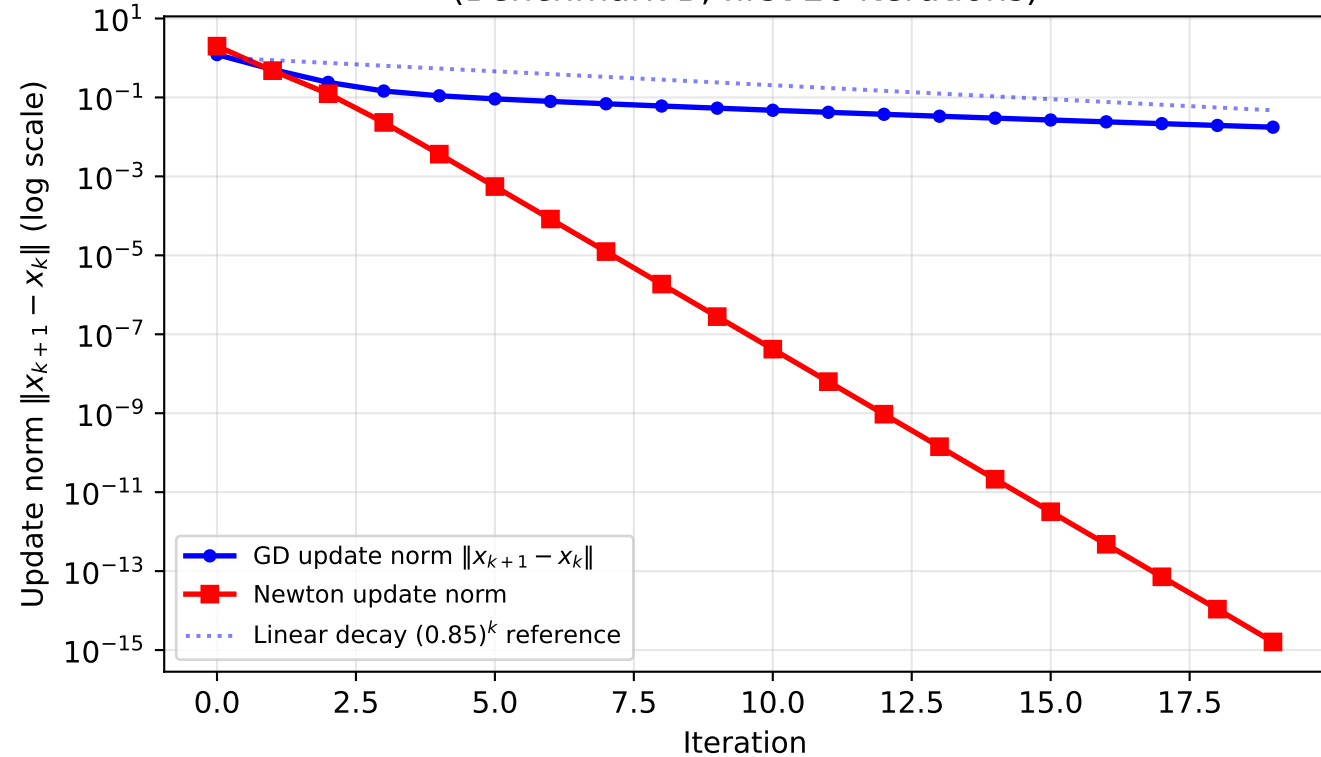
Q3: Update Norm Decay — Linear vs Rapid Convergence (Benchmark B, first 20 iterations)
