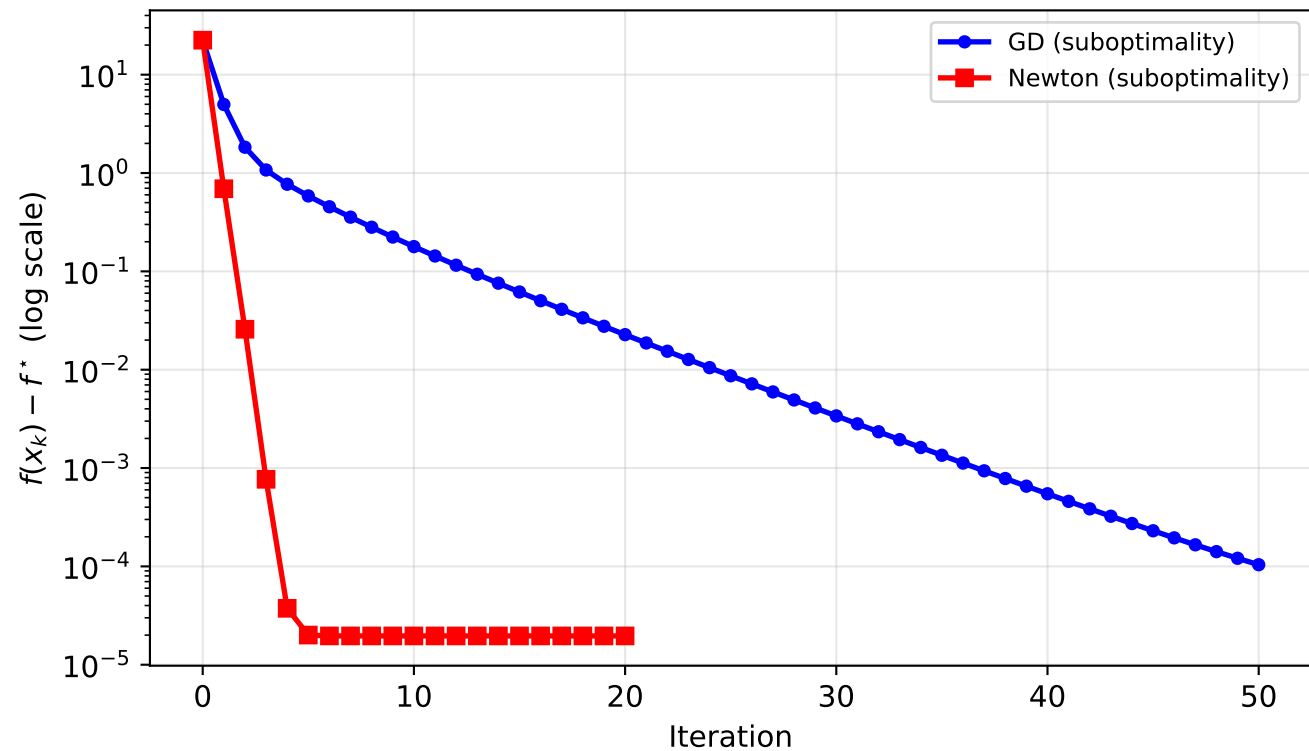
Q3: GD vs Newton's on Benchmark B (suboptimality f(x_k) - f^* )
