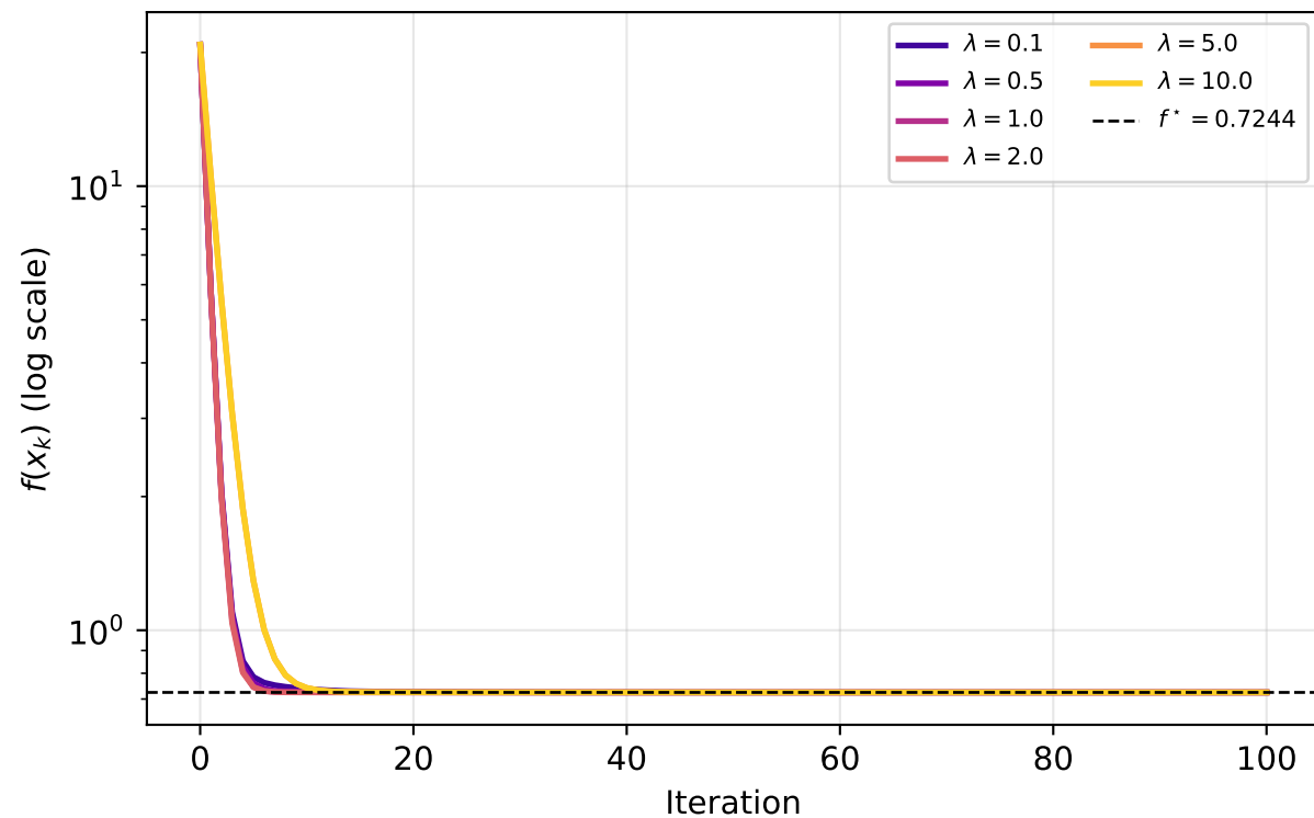
Q5: Penalty Method — Effect of \lambda on Convergence
