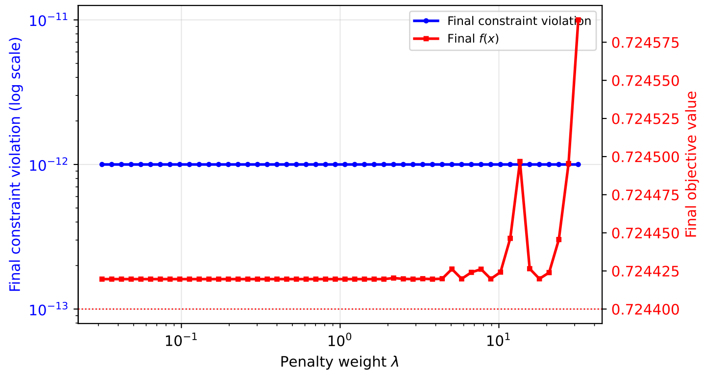
Q5: Penalty Method Trade-off ( \lambda effect on feasibility vs. optimality)
