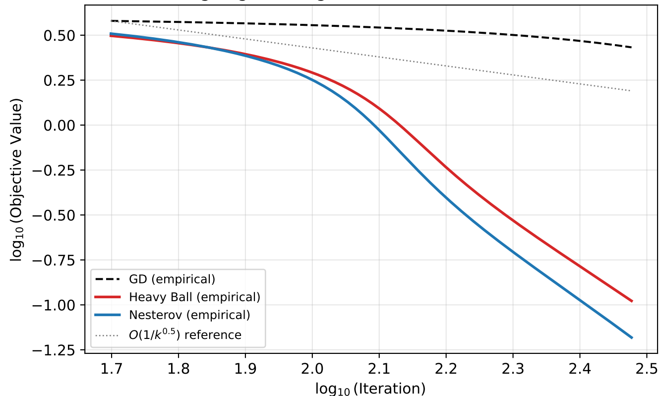
Log-Log Convergence Profile on Rosenbrock
