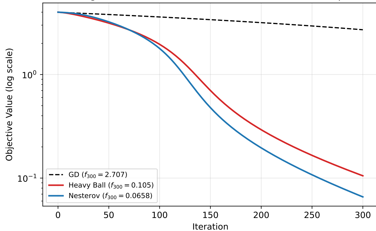
Convergence on Rosenbrock: Momentum Methods Compared
