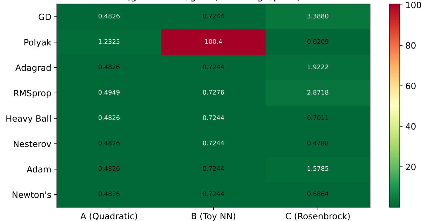
Final Objective Values After 150 Iterations (green=low/good, red=high/poor)
