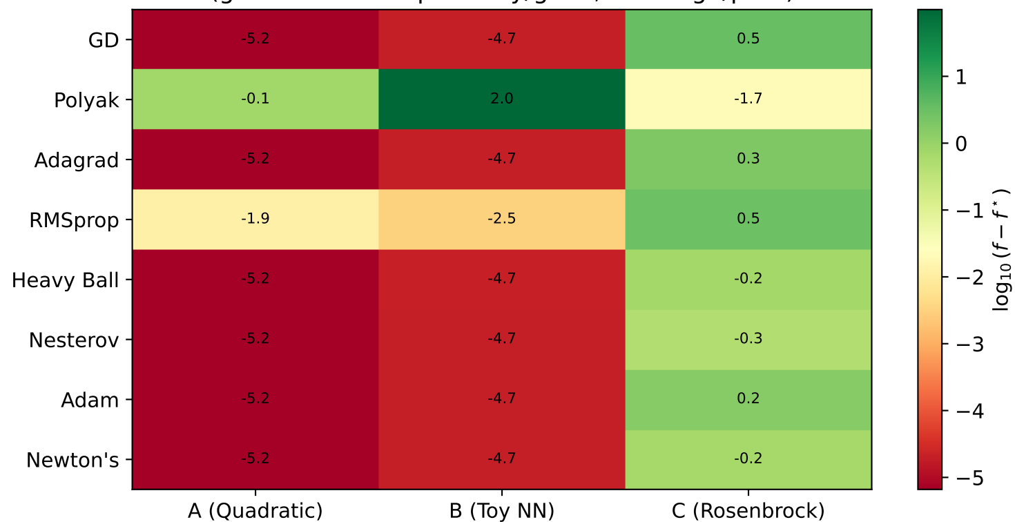
\log_{10}(f - f^*) After 150 Iterations (green=low suboptimality/good, red=high/poor)
