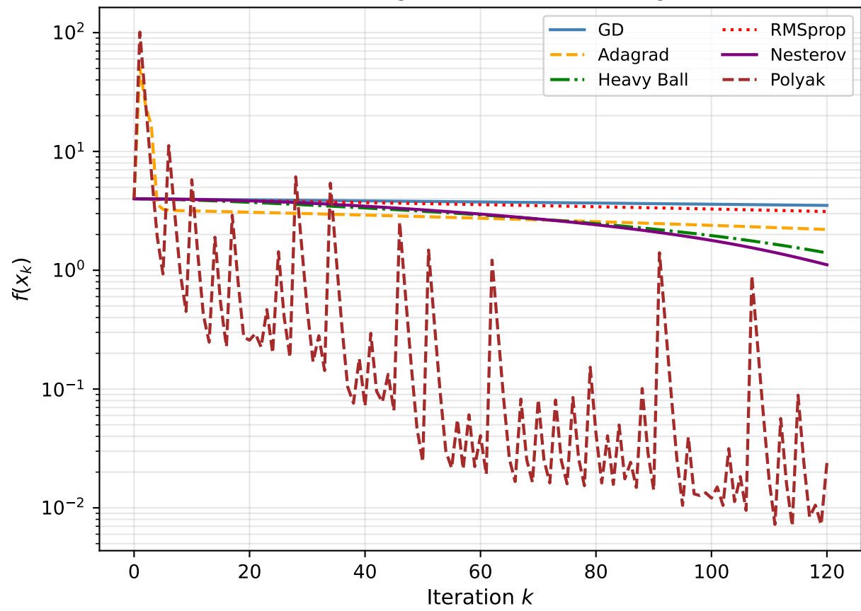
Q1 Convergence (120 iters, semi-log)
