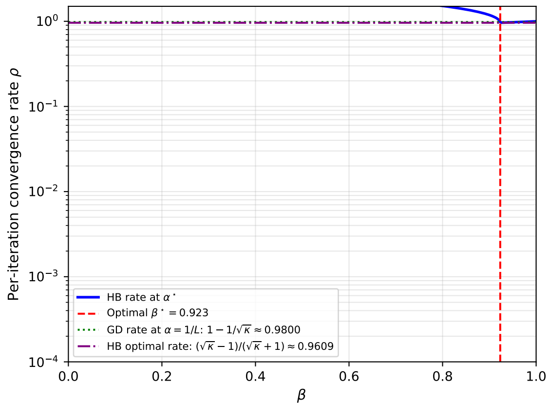
HB Rate vs \beta at \alpha = \alpha^* = 3.8388e - 03 (Rosenbrock, \kappa \approx 2510 )
