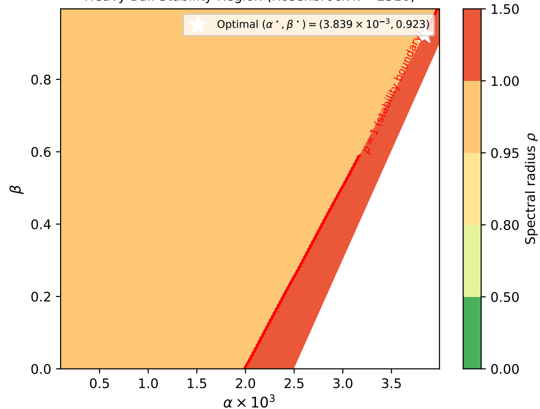
Heavy Ball Stability Region (Rosenbrock \kappa \approx 2510 )
