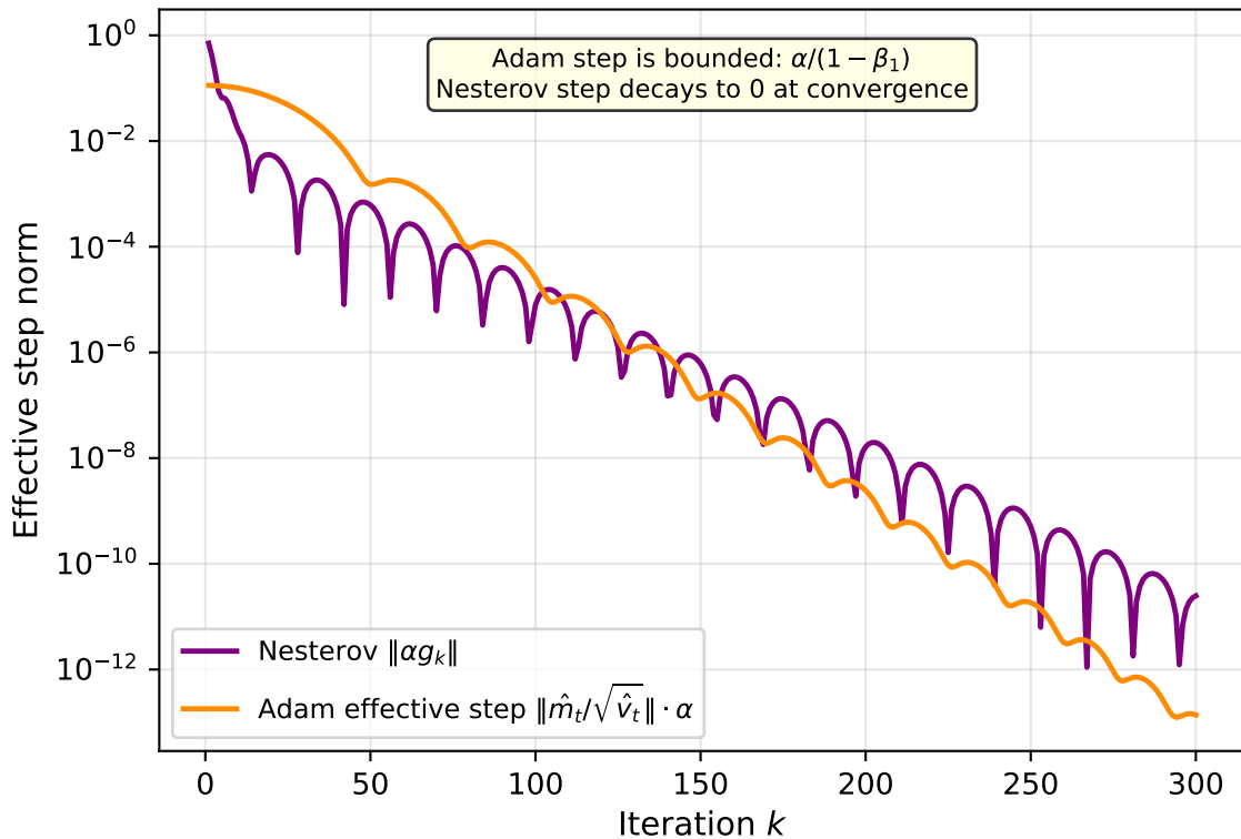
Effective Step Size: Nesterov vs Adam (Benchmark B)
