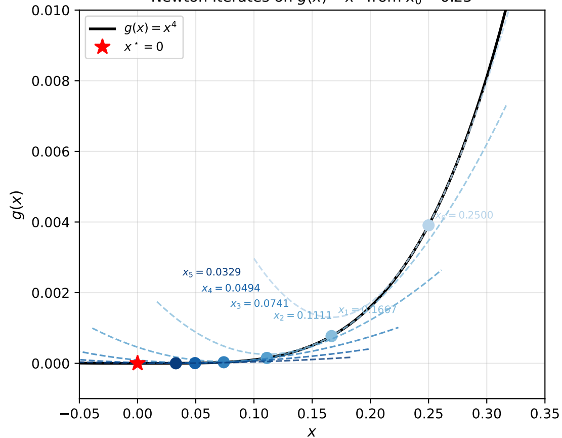
Newton Iterates on g(x) = x^4 from x_0 = 0.25
