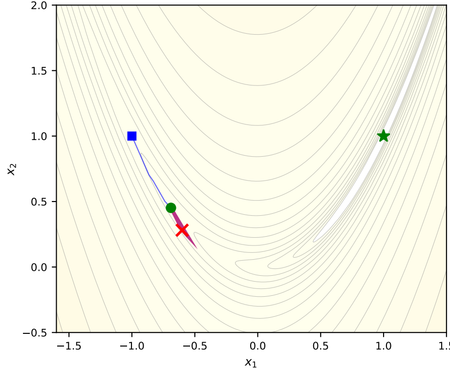
Iter 15: f_{\text{best}} = 2.9122
