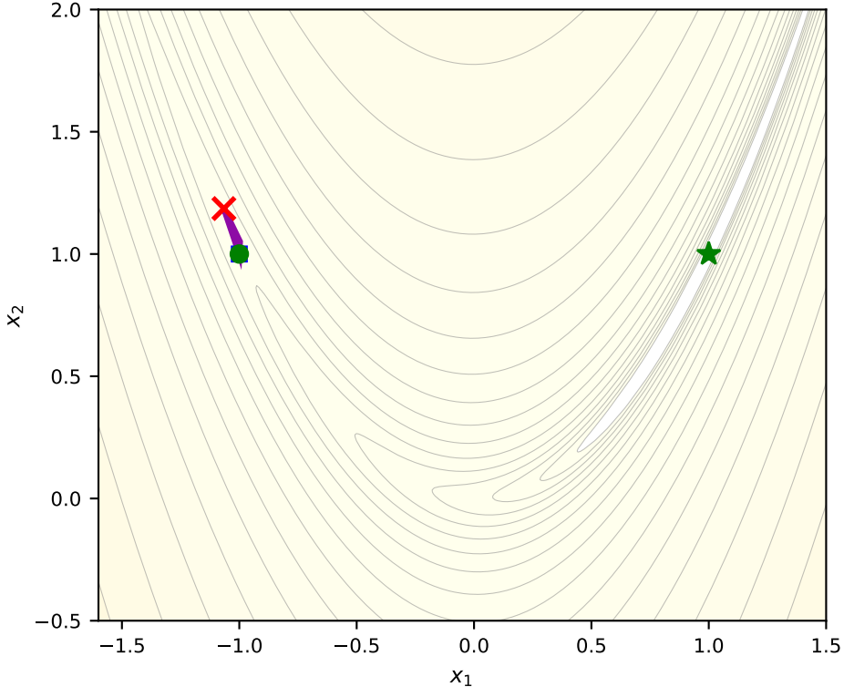
Iter 5: f_{\text{best}} = 4.0000
