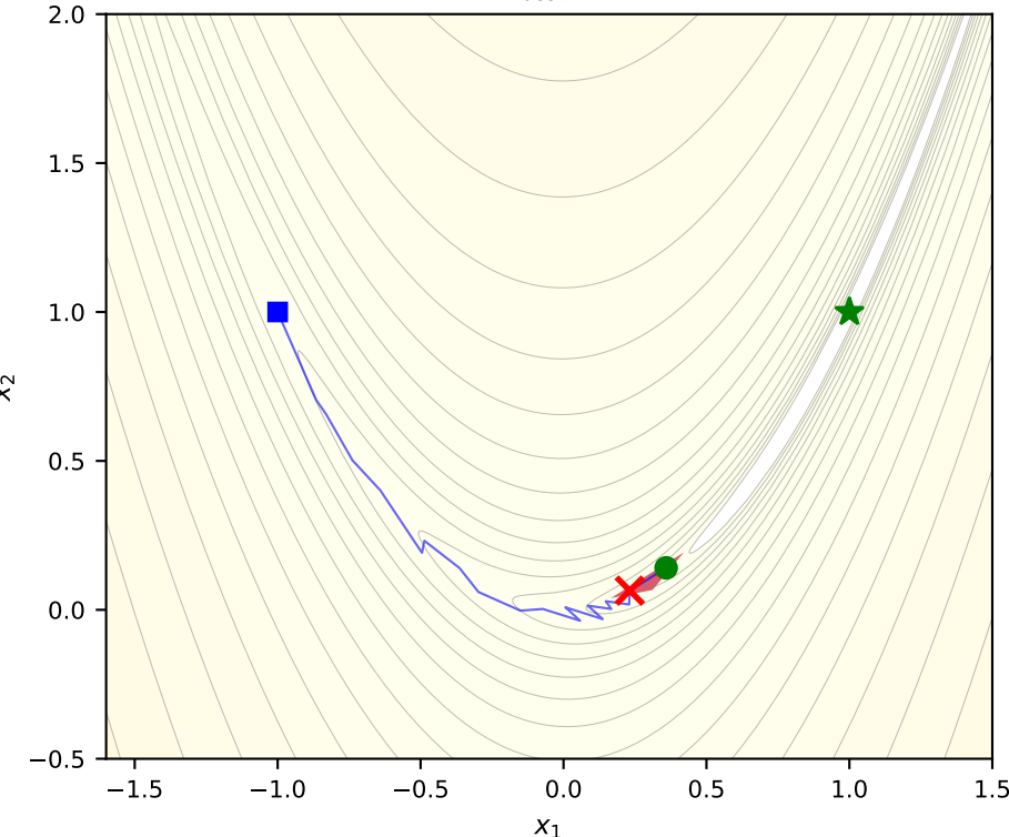
Iter 40: f_{\text{best}} = 0.4257
