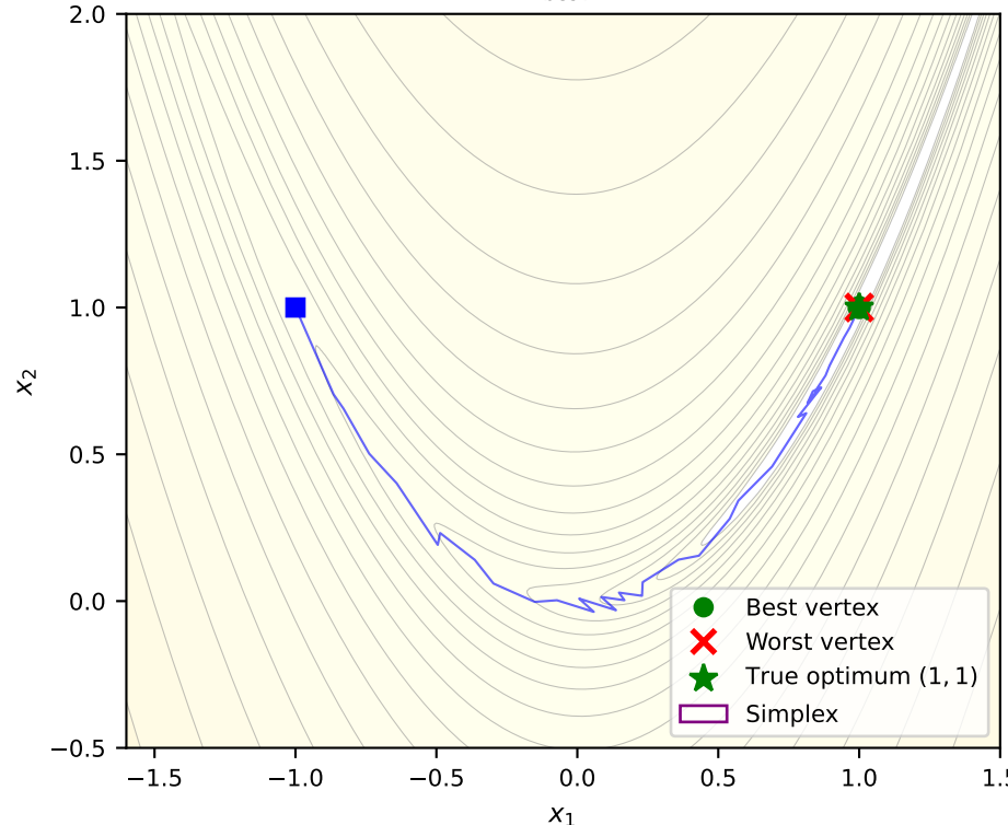
Iter 139: f_{\text{best}} = 0.0000
