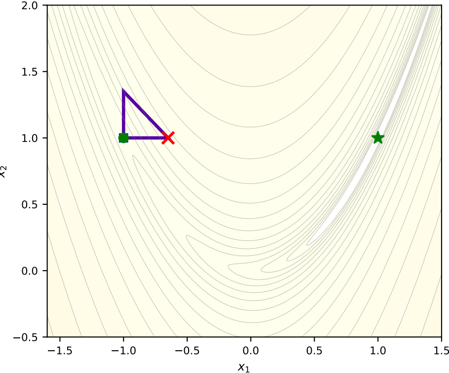
Iter 0: f_{\text{best}} = 4.0000
