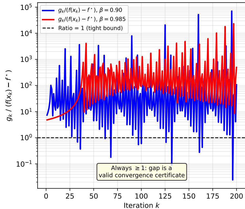
FW Gap Tightness: g_k \geq f(x_k) - f^*
