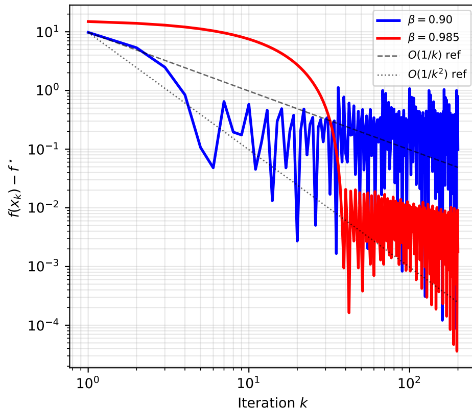
FW Convergence Rate (log--log)
