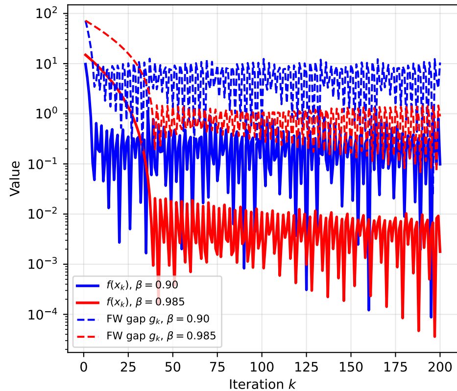
FW Objective and Gap (semi-log)
