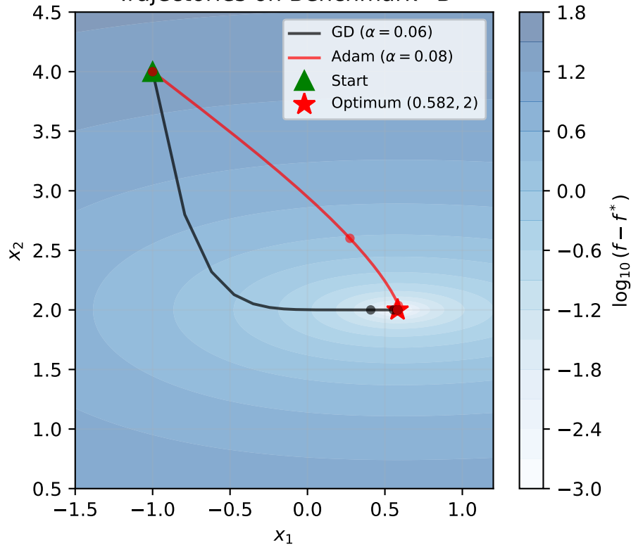
Trajectories on Benchmark~B
