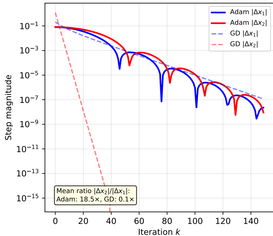
Per-Coordinate Step Sizes Adam vs GD
