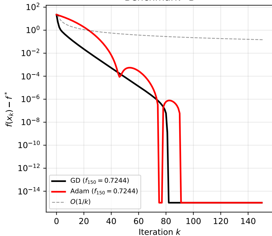
Convergence Comparison Benchmark~B
