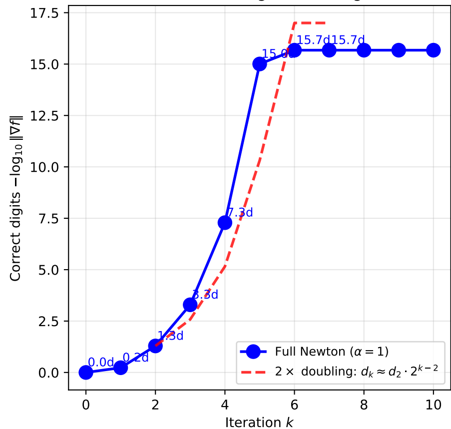
Full Newton ( \alpha = 1 ): Quadratic "Digits Doubling"
