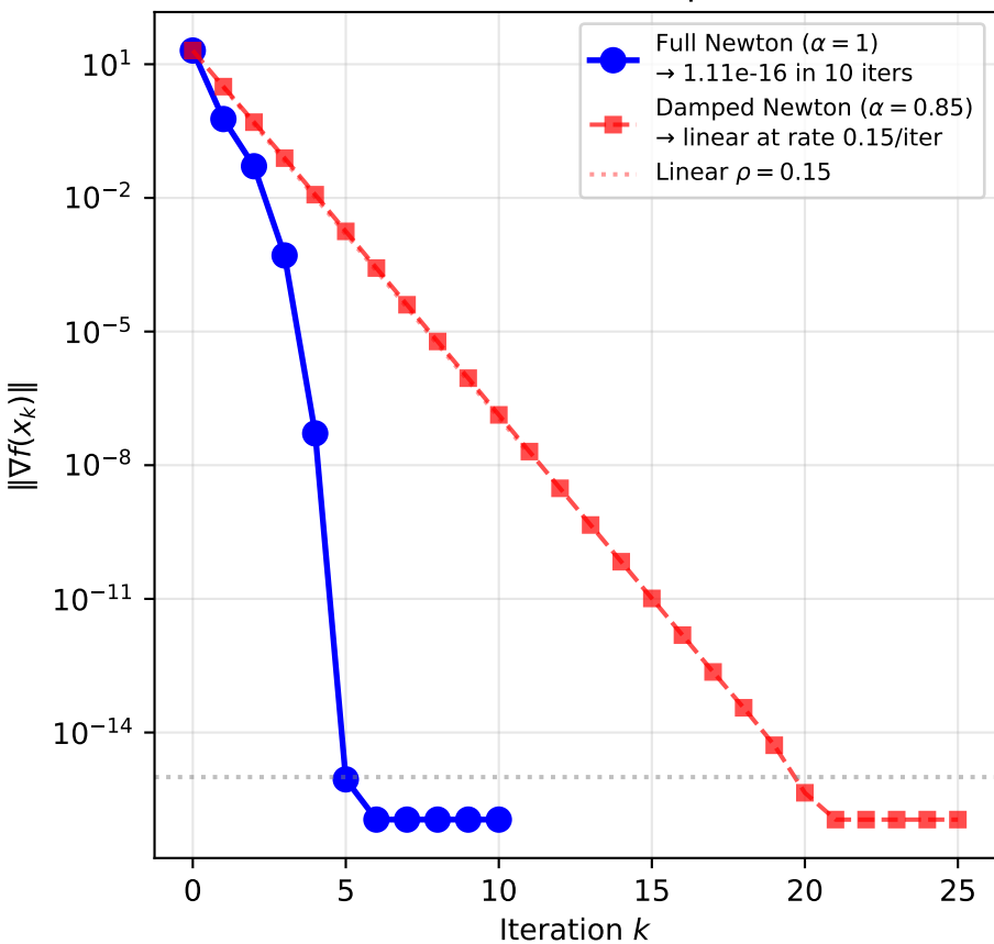
Full vs Damped Newton Gradient Norm Comparison
