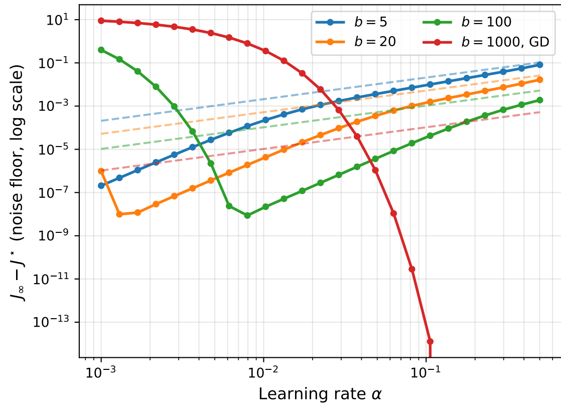
SGD Noise Floor: Theory vs Empirical (dashed = theory \alpha\sigma^2/2\mu b )
