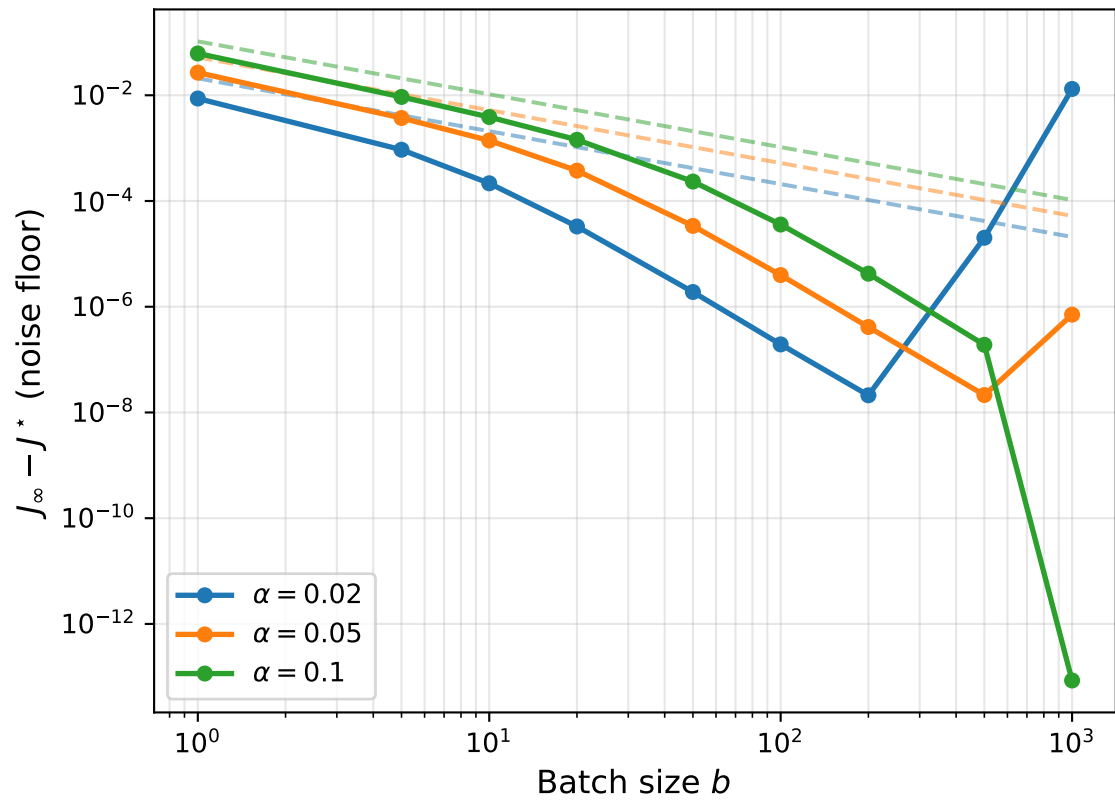
Noise Floor vs Batch Size (dashed = theory \alpha\sigma^2/2\mu b )
