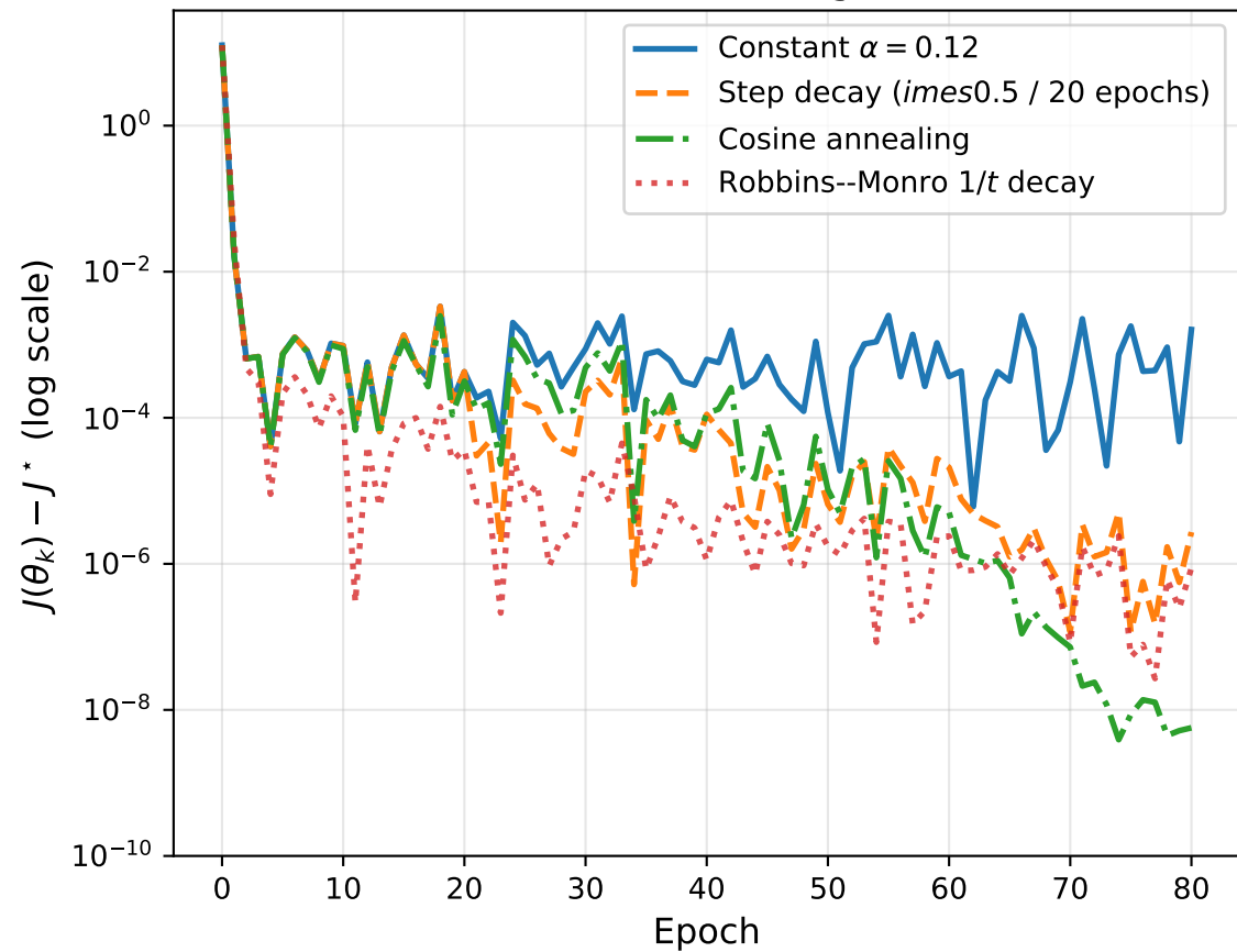
SGD on Benchmark A: Learning Rate Schedules
