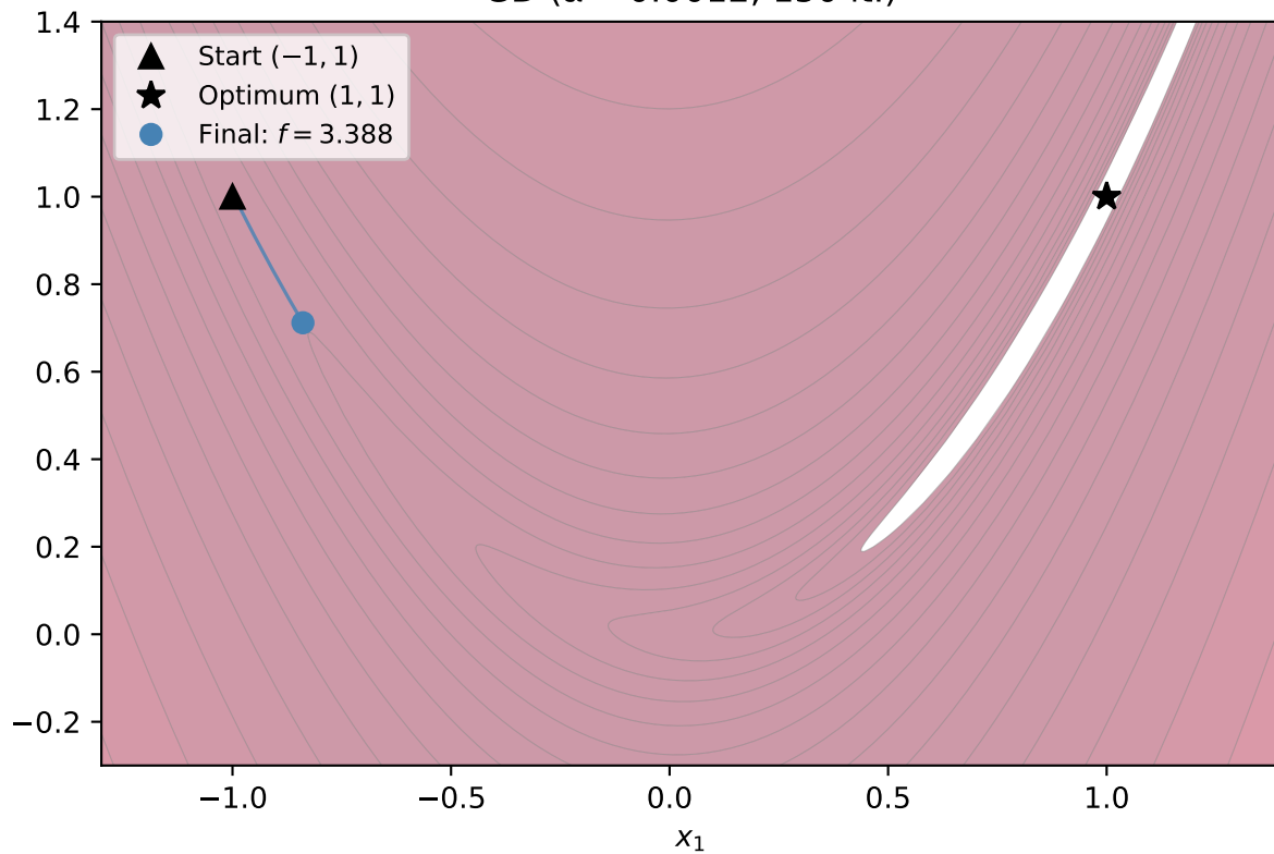
GD ( \alpha = 0.0012 , 150 it.)
