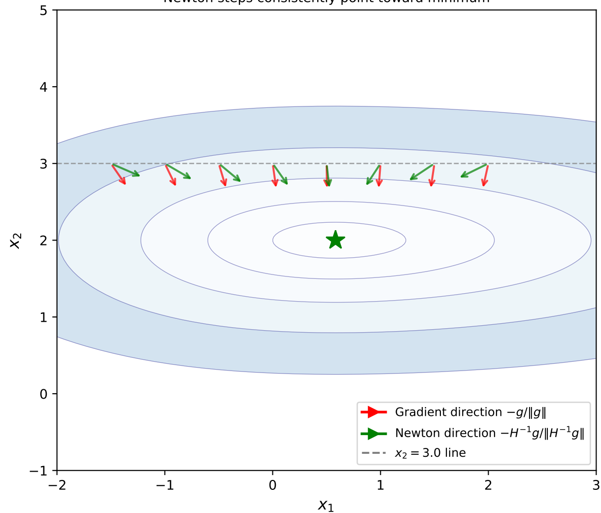
Systematic Curvature Correction: Newton steps consistently point toward minimum
