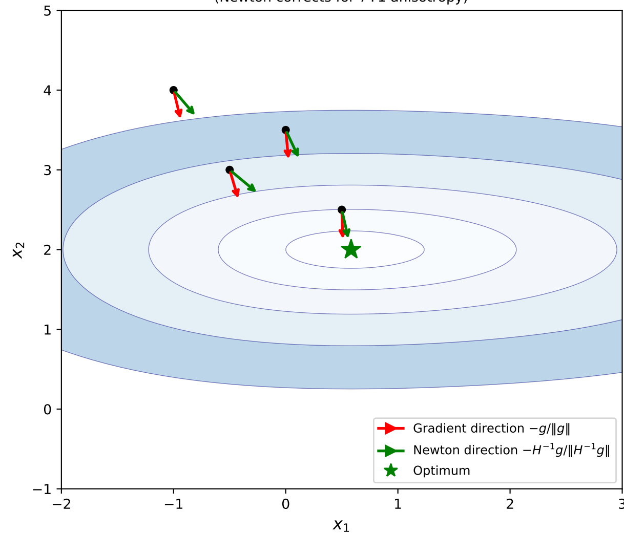
Gradient vs Newton Direction on Benchmark B (Newton corrects for 7 : 1 anisotropy)
