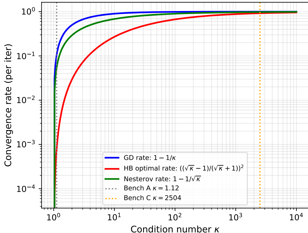
Convergence Rates vs. Condition Number
