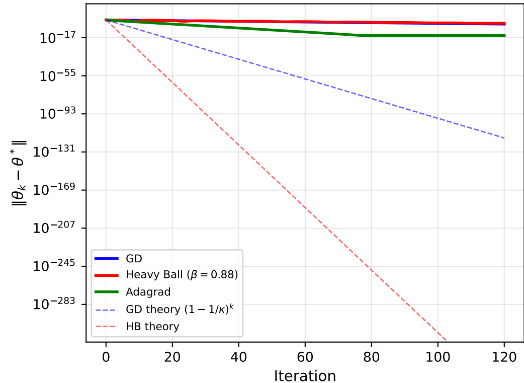
Benchmark A: Distance to Optimum
