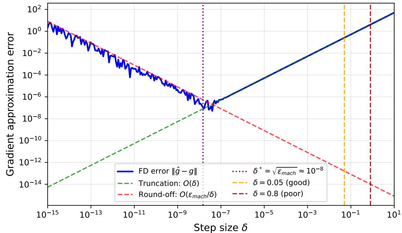
Finite Difference Error vs. Step Size (Benchmark B, x_0 = (-1, 4) )
