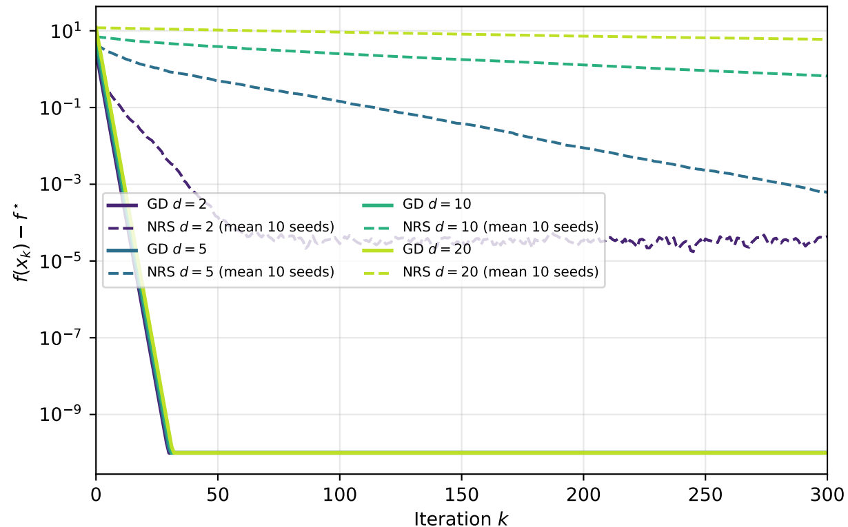
GD vs Nesterov Random Search Convergence for Various Dimensions d
