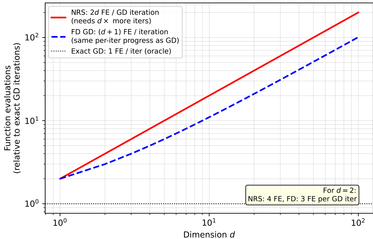
Oracle Complexity: FE to Match Exact GD ( \kappa = 5 , ignore log factors)
