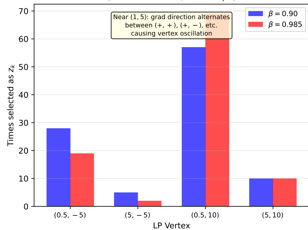
LP Vertex Selection Frequency (100 FW iterations, interior opt.)
