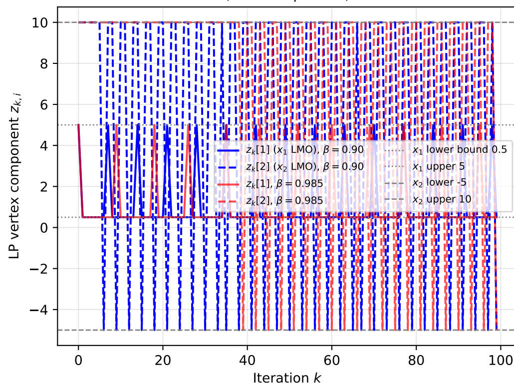
Frank--Wolfe LP Vertex z_k vs Iteration (Interior Optimum)
