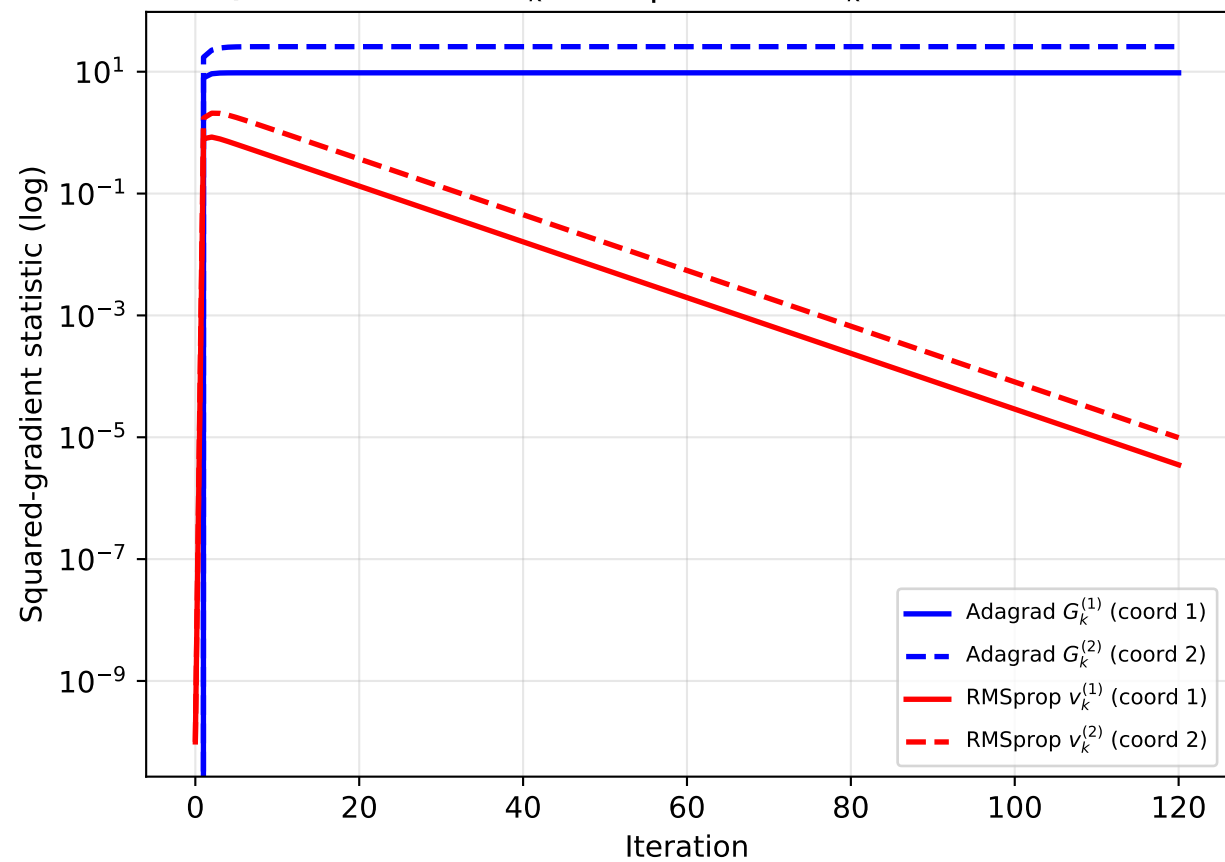
Q1: Cumulative G_k vs Exponential v_k — Benchmark A
