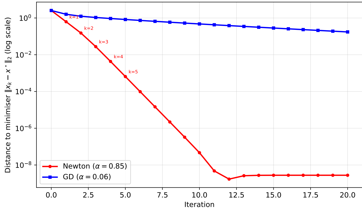
Q3: Distance to Minimiser x^* = (0.582, 2.0) — Benchmark B
