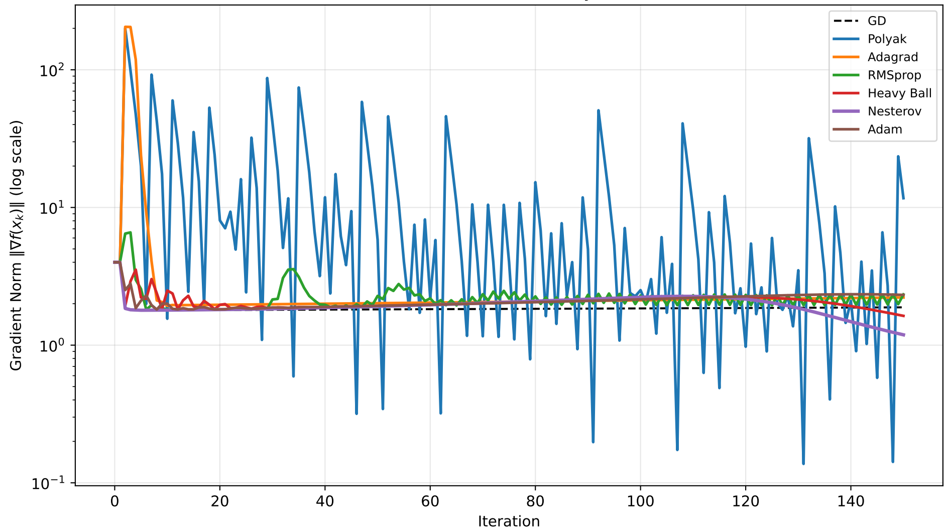
Benchmark C (Rosenbrock): Gradient Norm Decay — All Methods (150 iterations)
