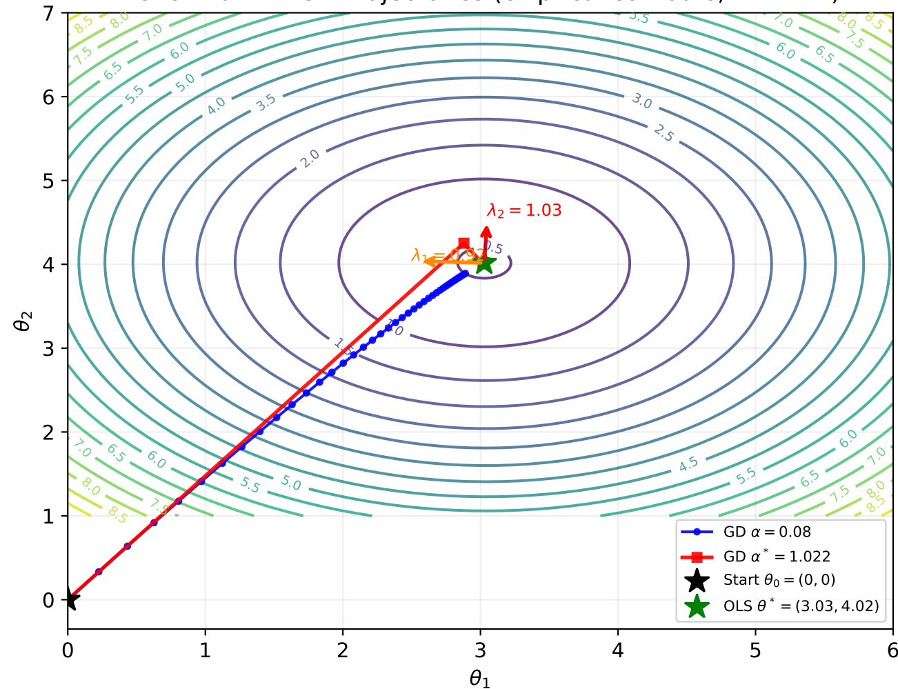
Benchmark A: GD Trajectories (elliptical contours, \kappa \approx 1.12 )
