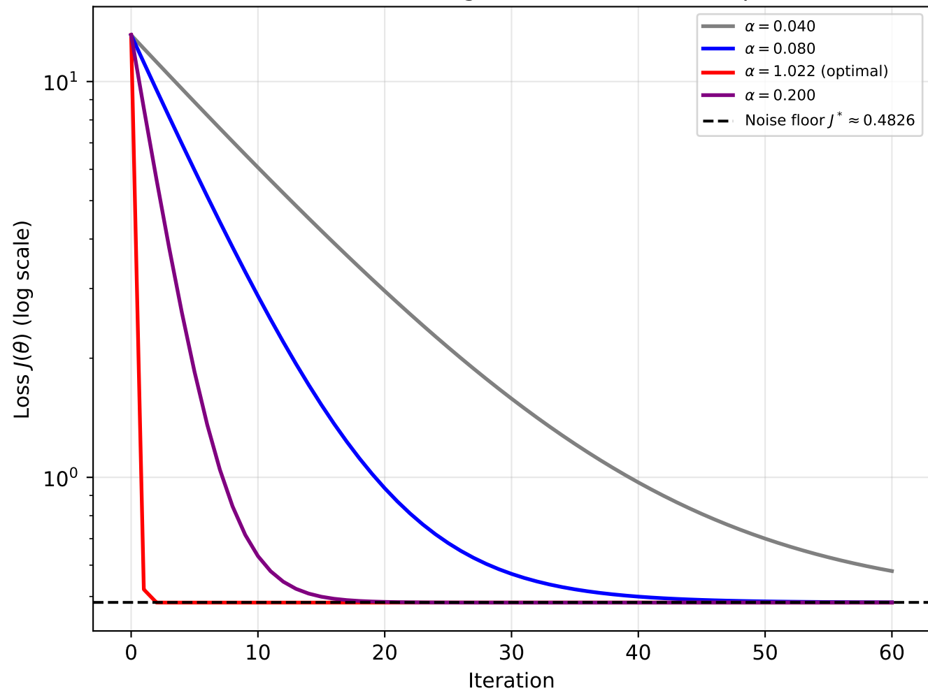
Benchmark A: Convergence for Different Step Sizes
