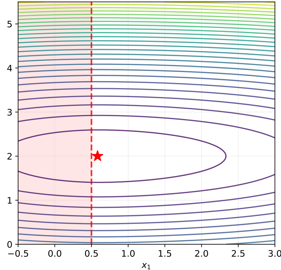
\lambda = 0.15
