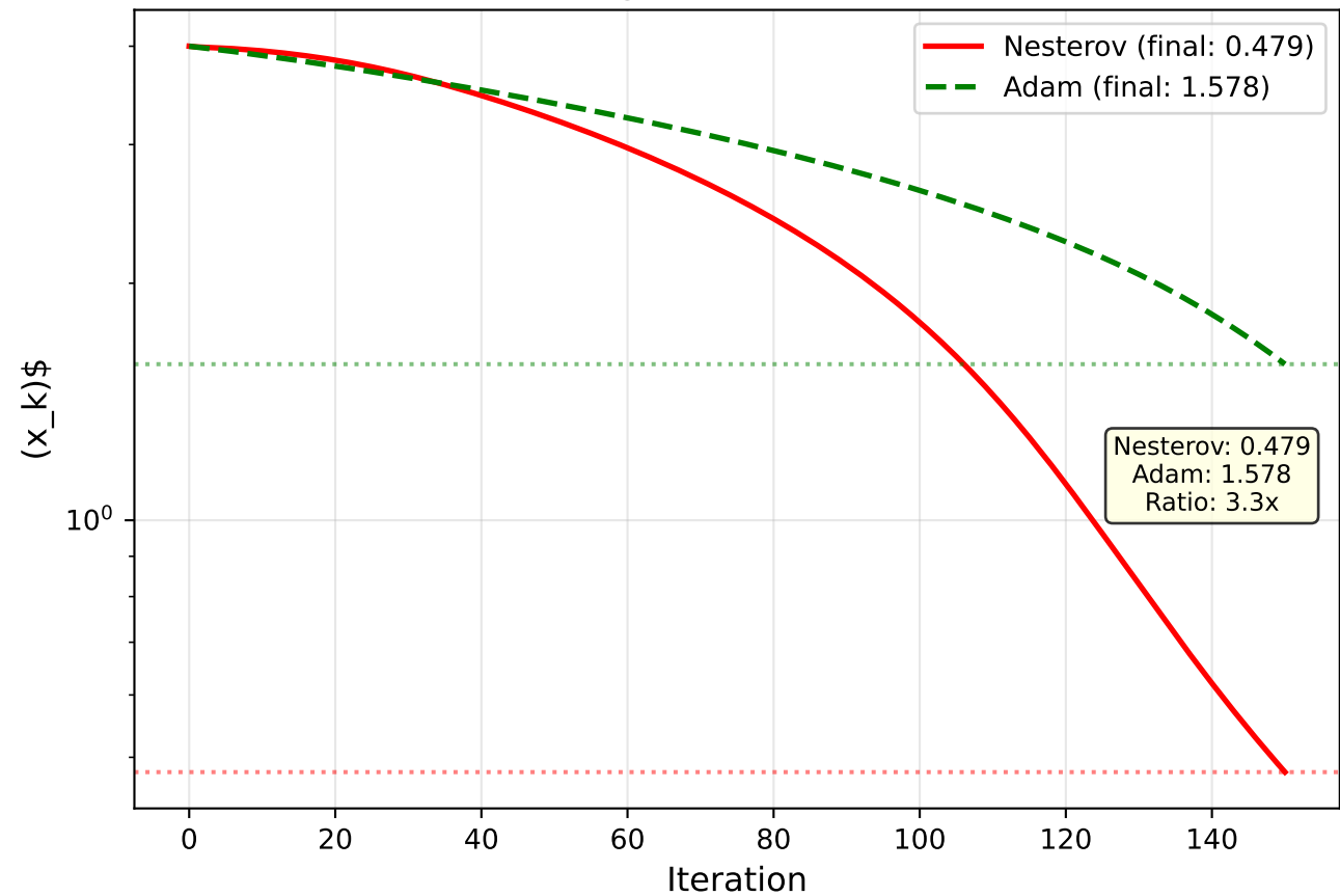
Convergence on Rosenbrock
