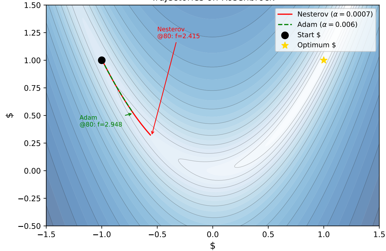
Trajectories on Rosenbrock
