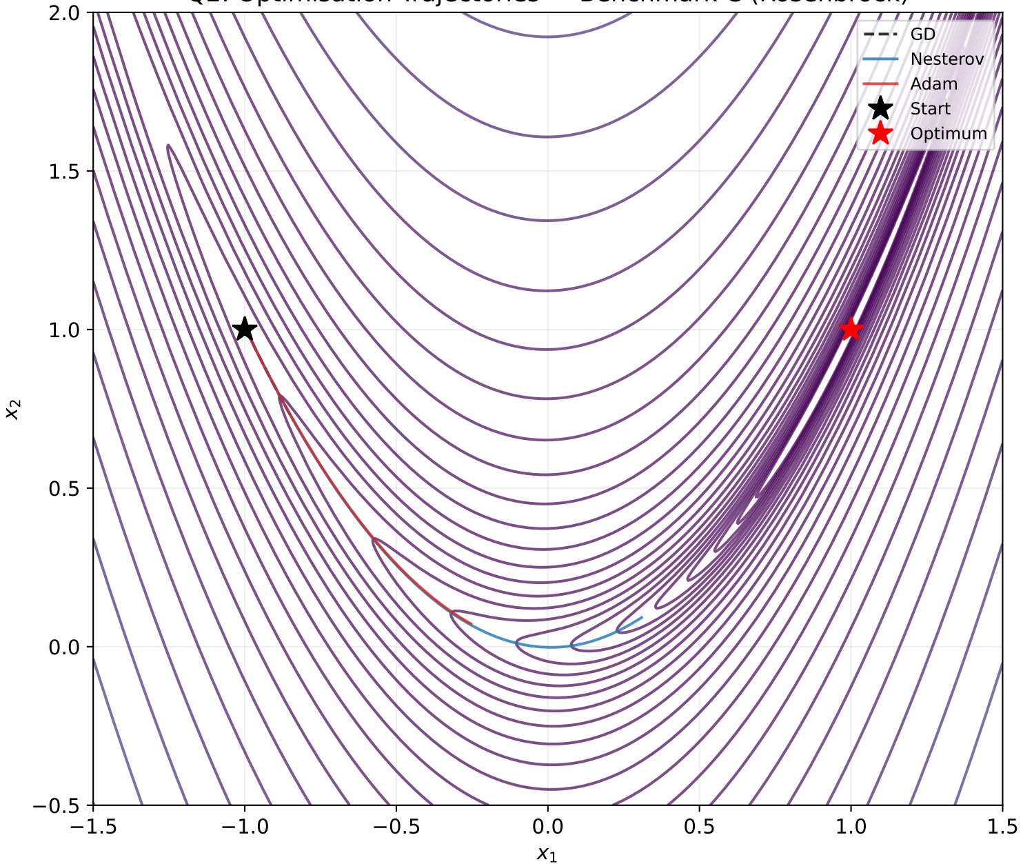
Q2: Optimisation Trajectories — Benchmark C (Rosenbrock)
