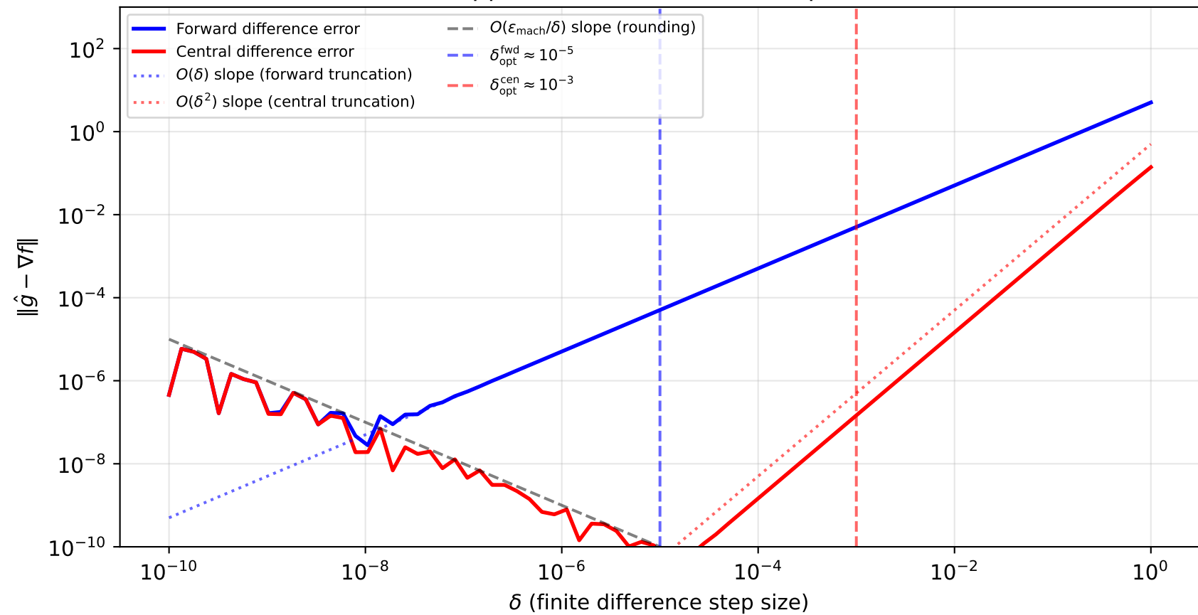
Finite Difference Approximation Error vs. Step Size (Benchmark B)
