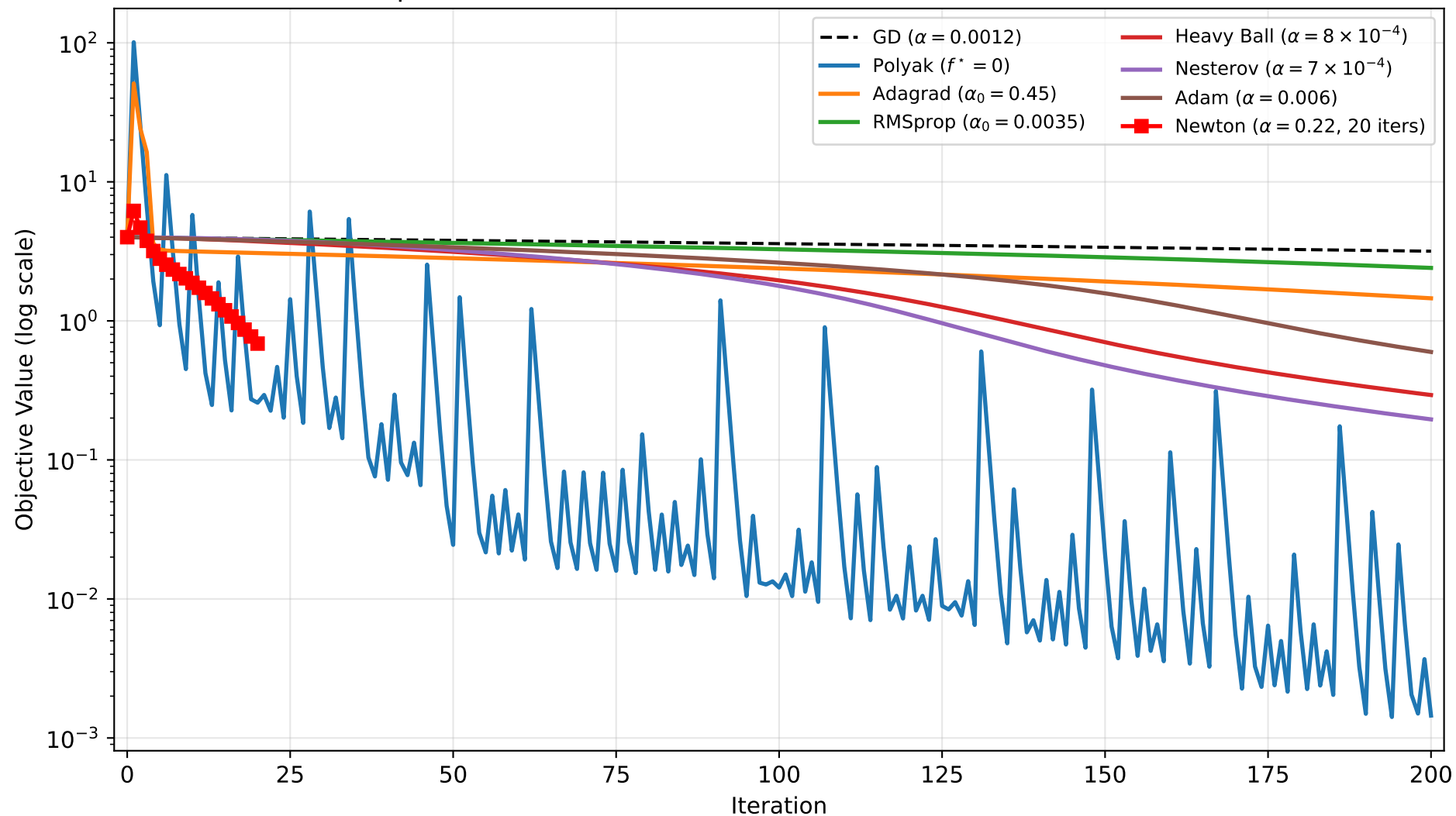
Grand Comparison: All Gradient-Based Methods on Benchmark C (Rosenbrock)
