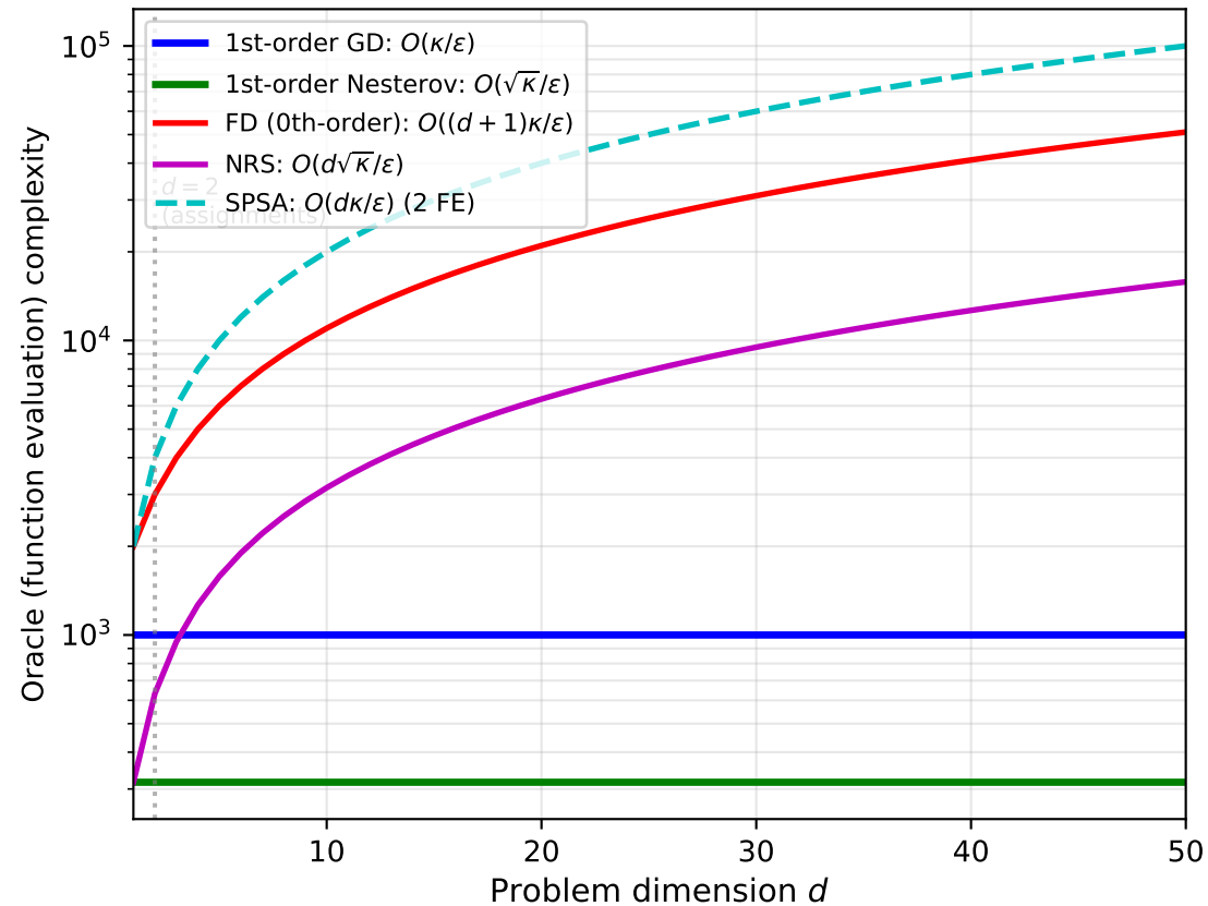
Oracle Complexity vs Dimension ( \kappa = 10.0, \varepsilon = 0.01 )
