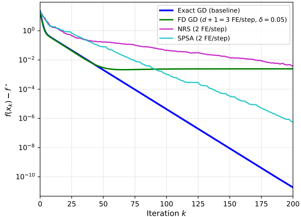
SPSA vs NRS vs FD on Benchmark B ( d = 2, \kappa = 6.9 )
