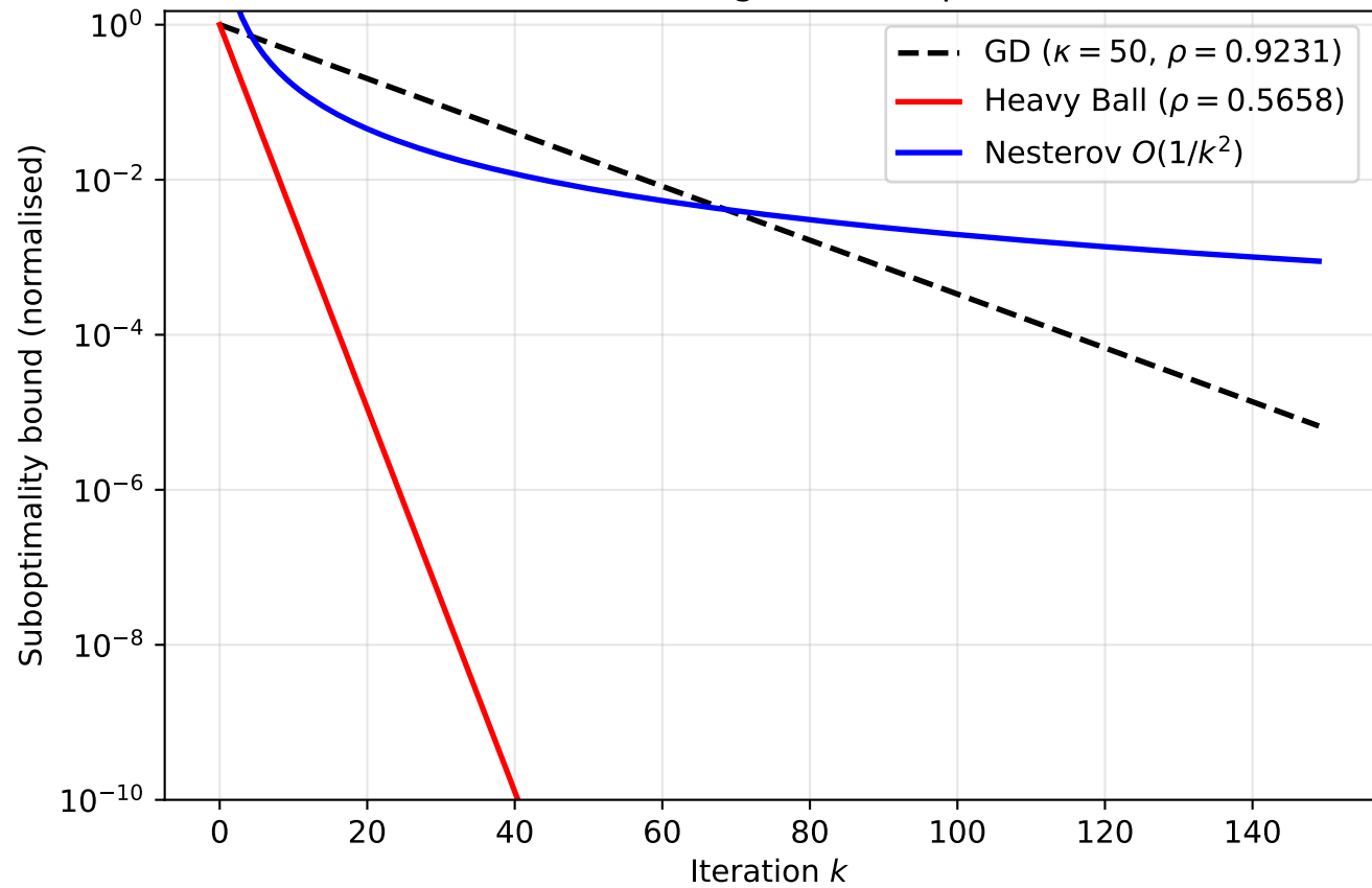
Q2: Theoretical Convergence Comparison ( \kappa = 50 )
