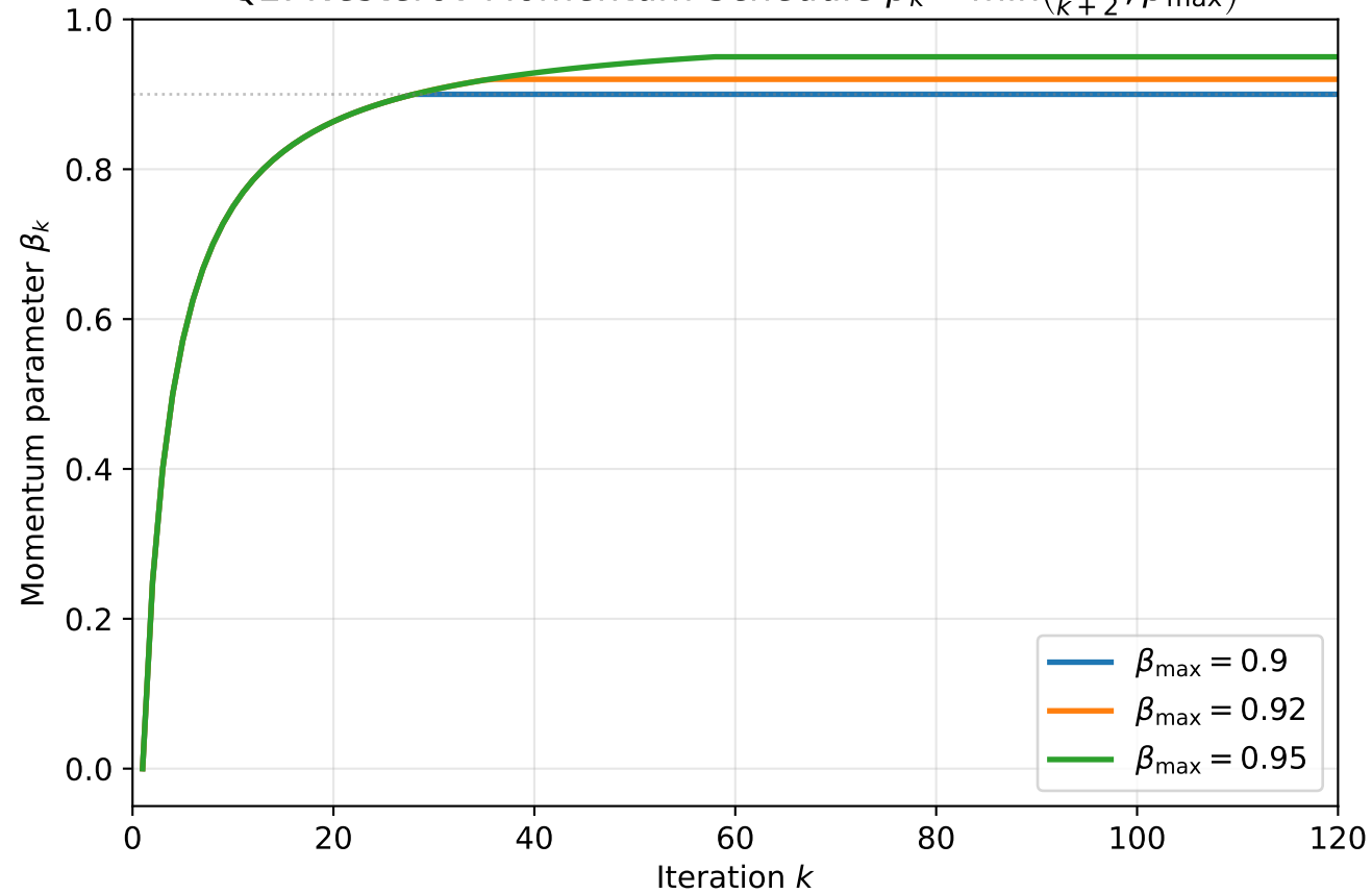
Q2: Nesterov Momentum Schedule \beta_k = \min(\frac{k-1}{k+2}, \beta_{\max})
