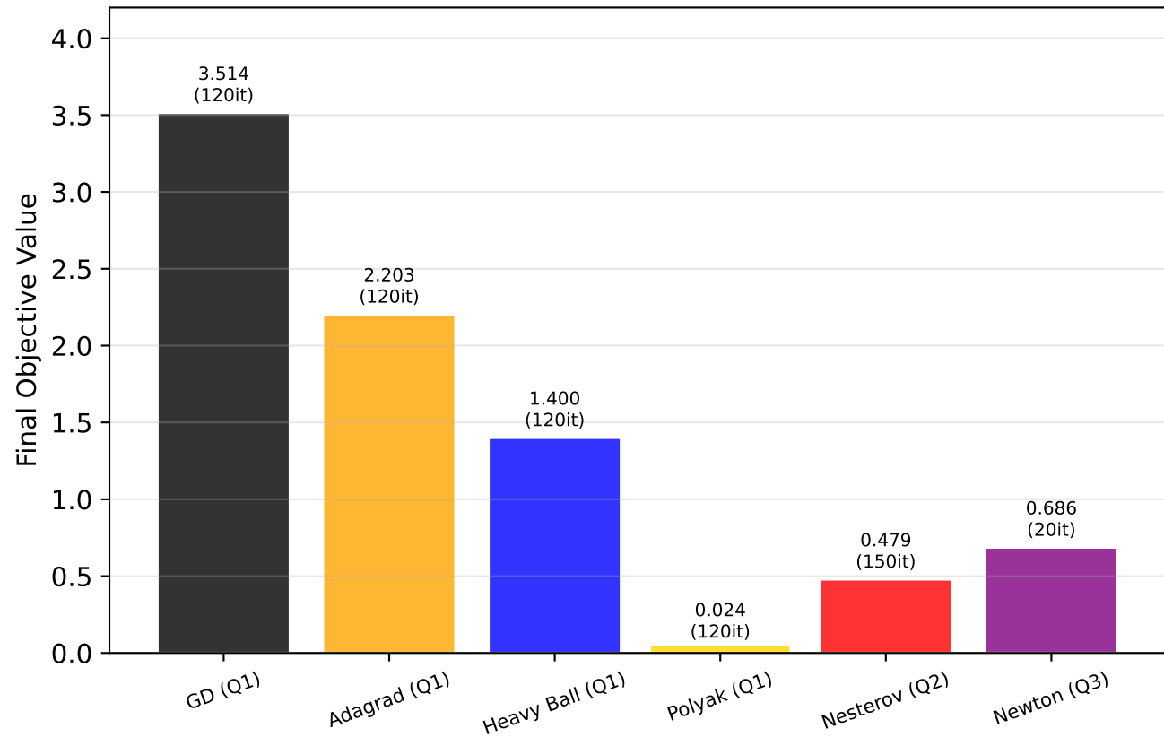
Final f on Rosenbrock (gold = best; budget shown)
