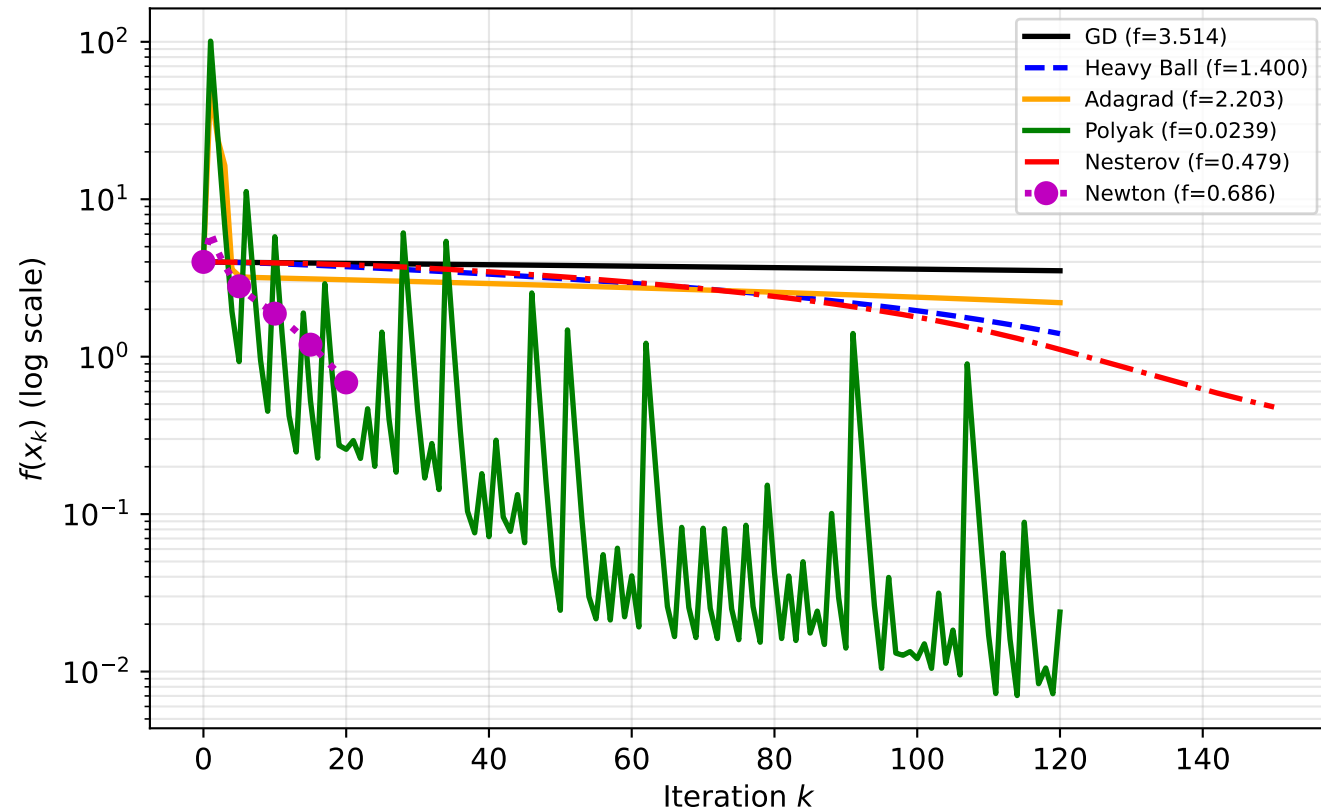
Benchmark C (Rosenbrock): All Methods Compared
